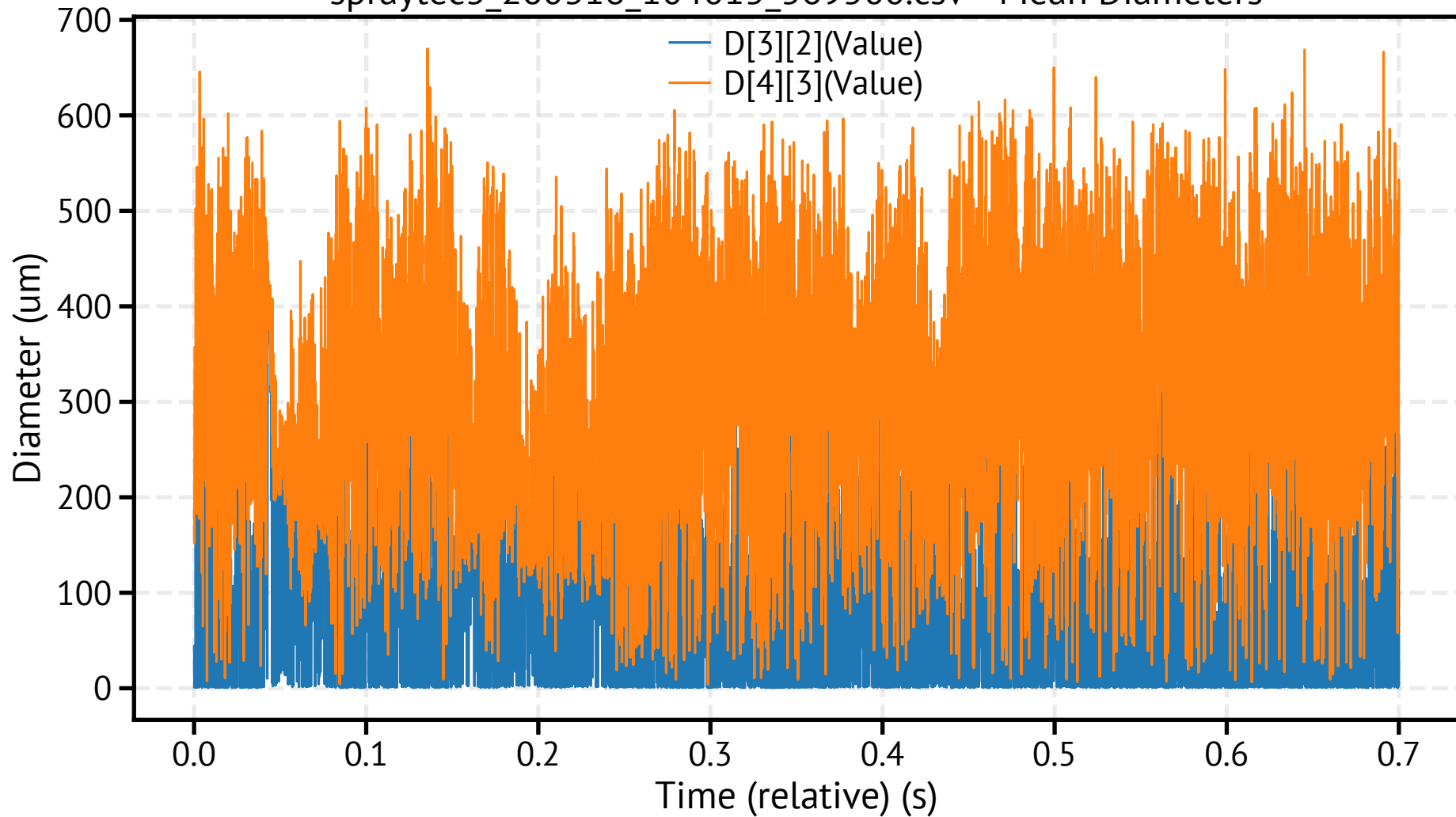
spraytec3_260318_104015_569500.csv - Mean Diameters
