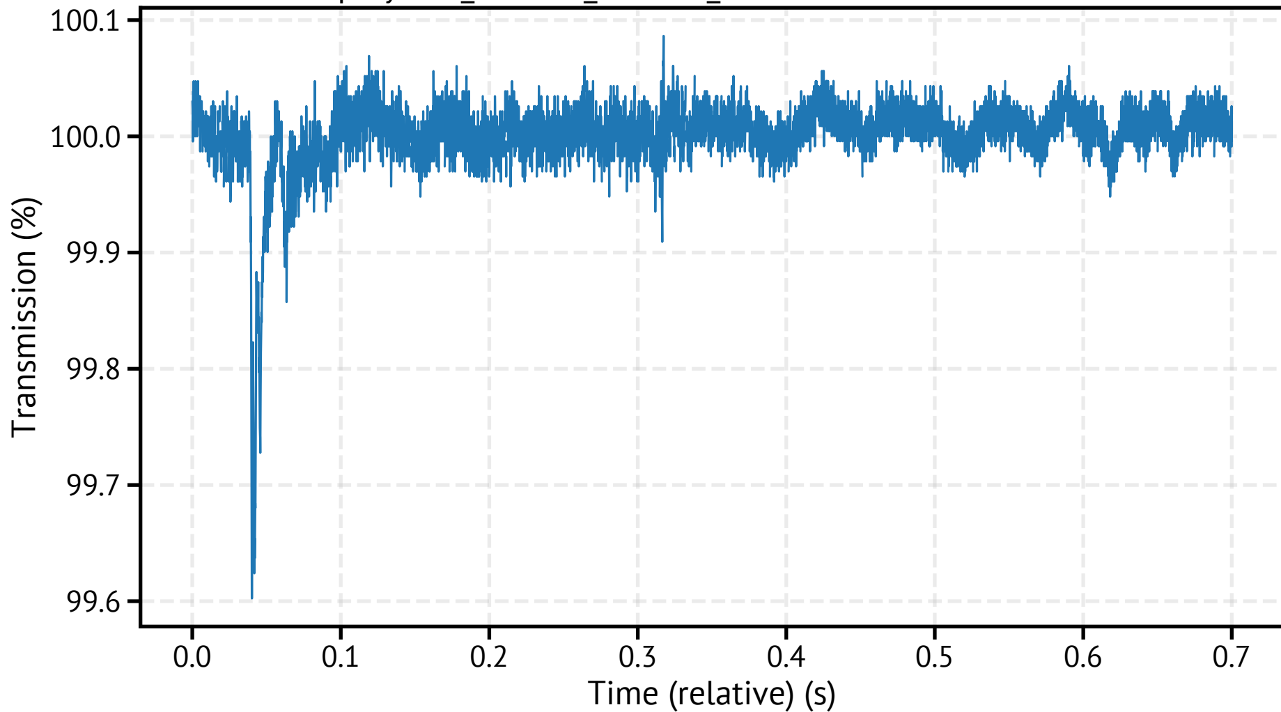
spraytec4_260318_104113_253000.csv - Transmission
