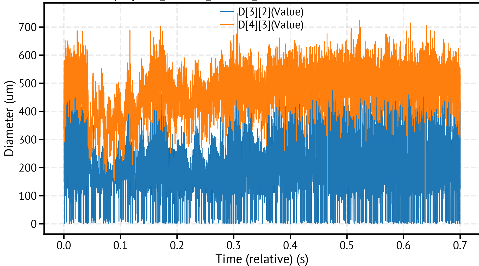
spraytec7_260318_104406_193000.csv - Mean Diameters
