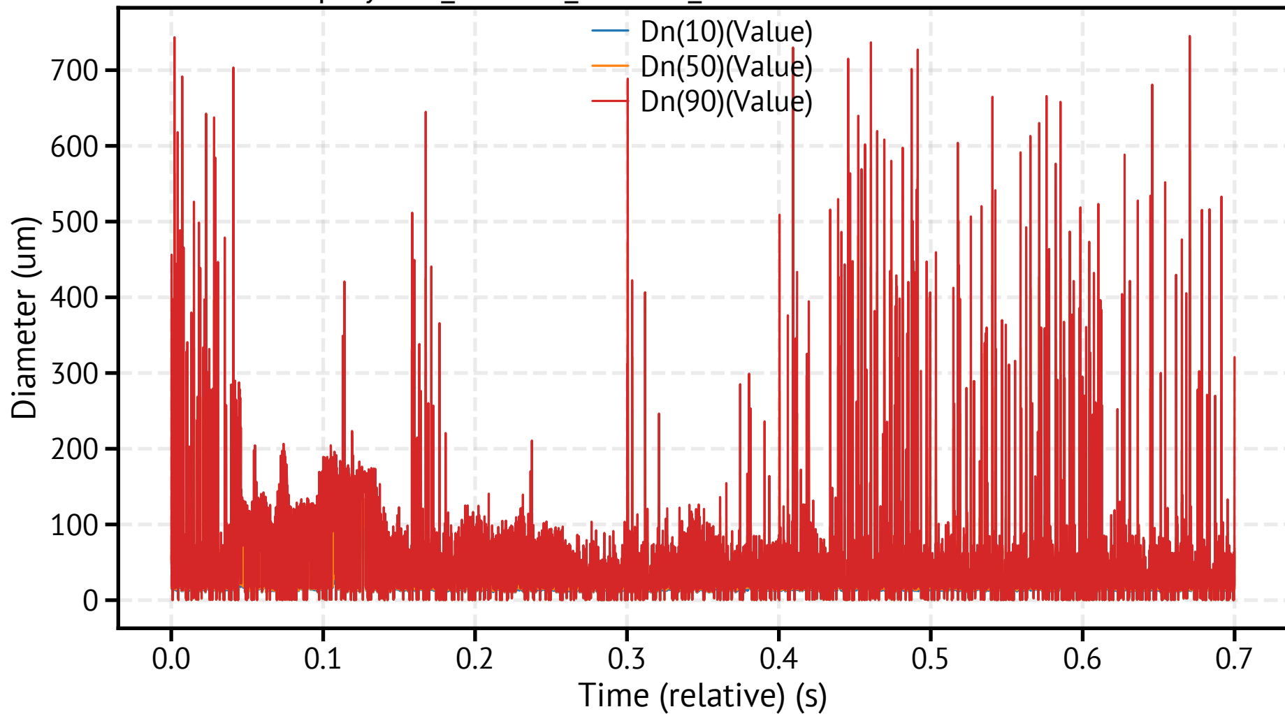
spraytec7_260318_104406_193000.csv - Dn Percentiles
