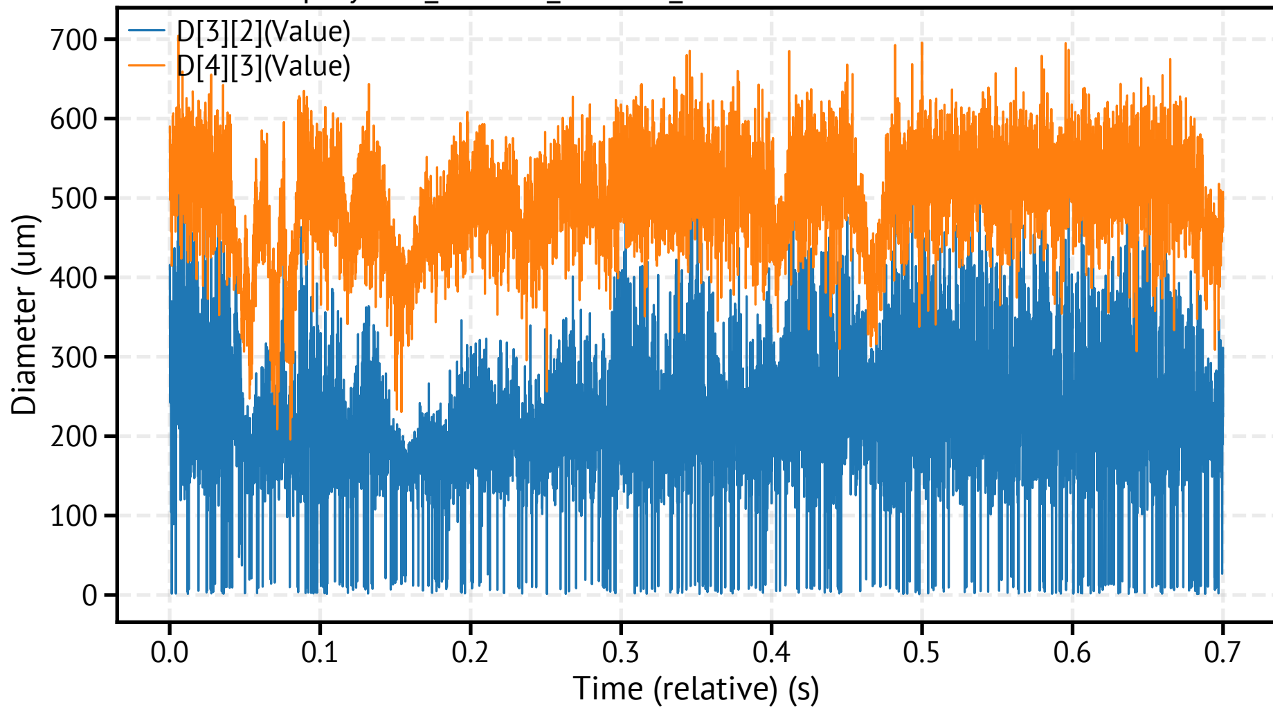
spraytec9_260318_104601_470200.csv - Mean Diameters
