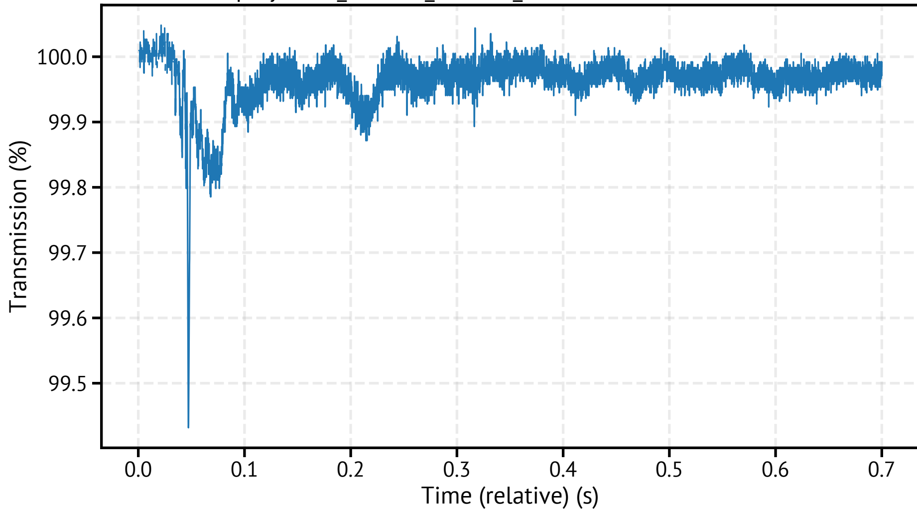
spraytec10_260318_111227_060600.csv - Transmission
