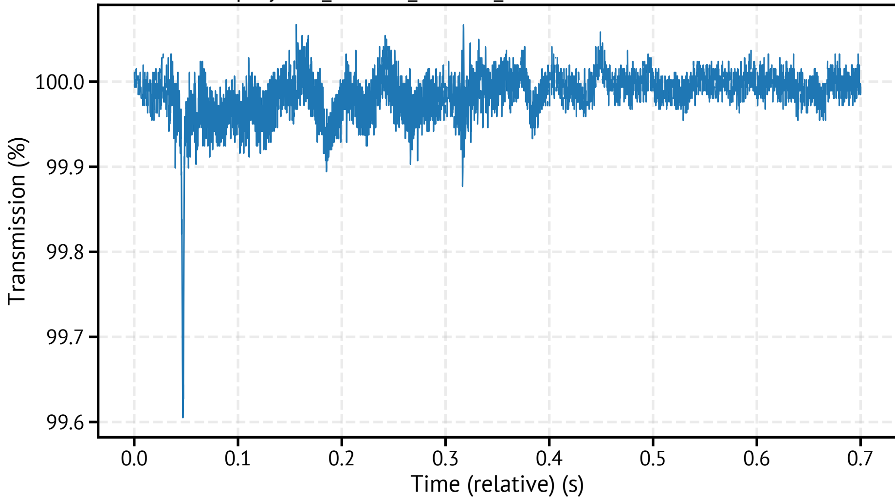
spraytec2_260318_110445_965600.csv - Transmission
