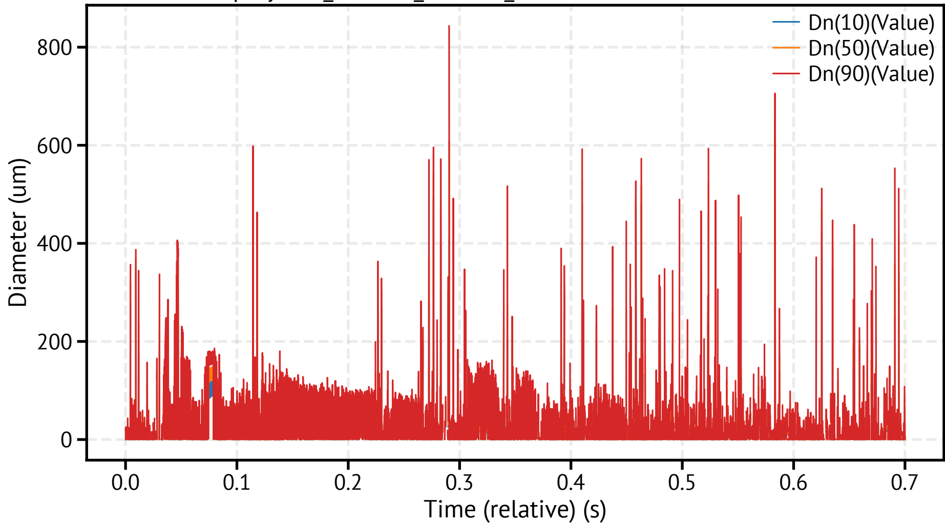
spraytec3_260318_110543_583400.csv - Dn Percentiles
