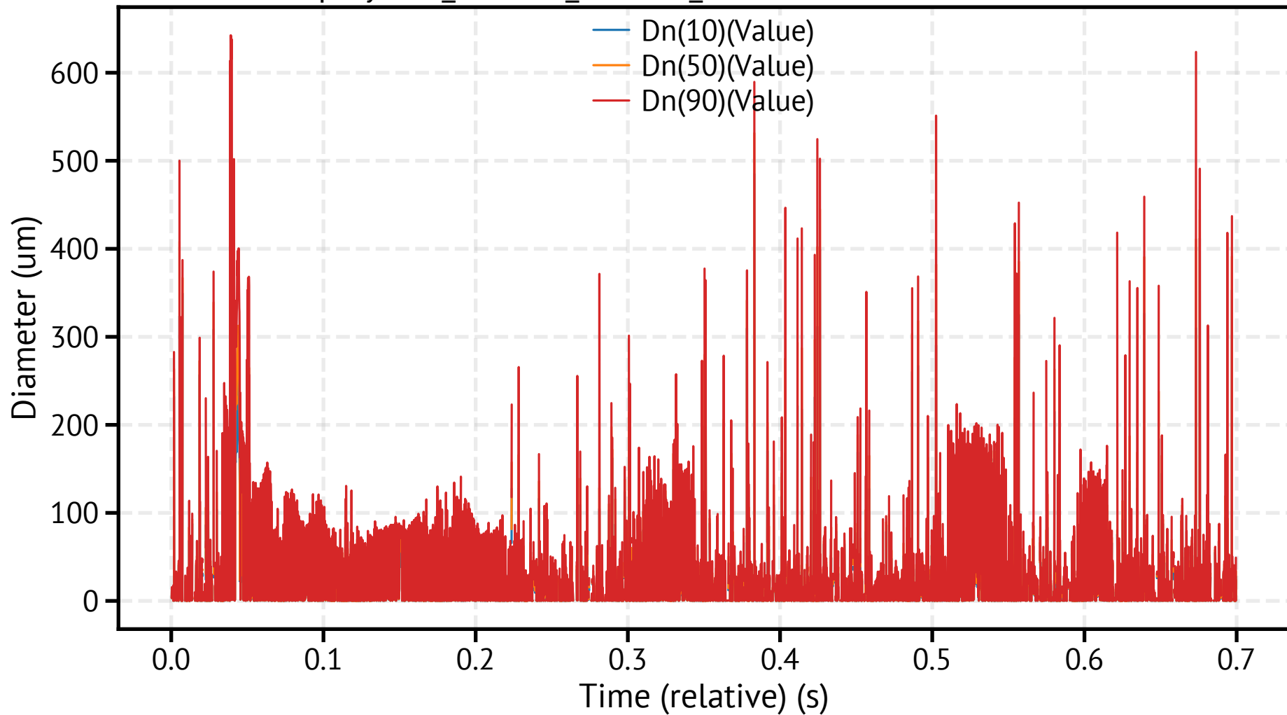
spraytec4_260318_110641_199800.csv - Dn Percentiles
