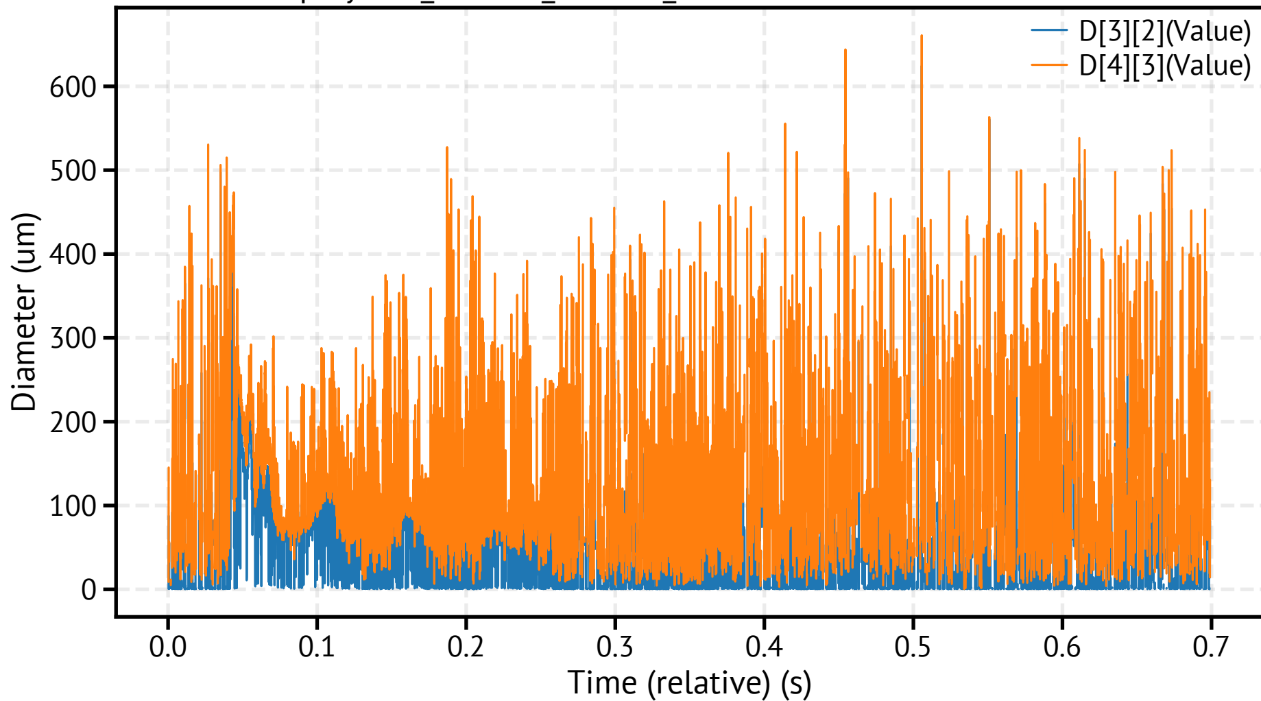
spraytec5_260318_110738_866400.csv - Mean Diameters
