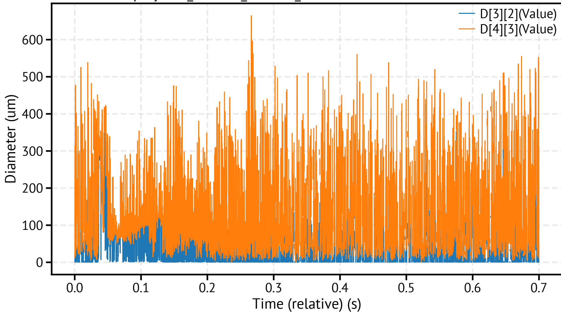
spraytec6_260318_110836_412500.csv - Mean Diameters
