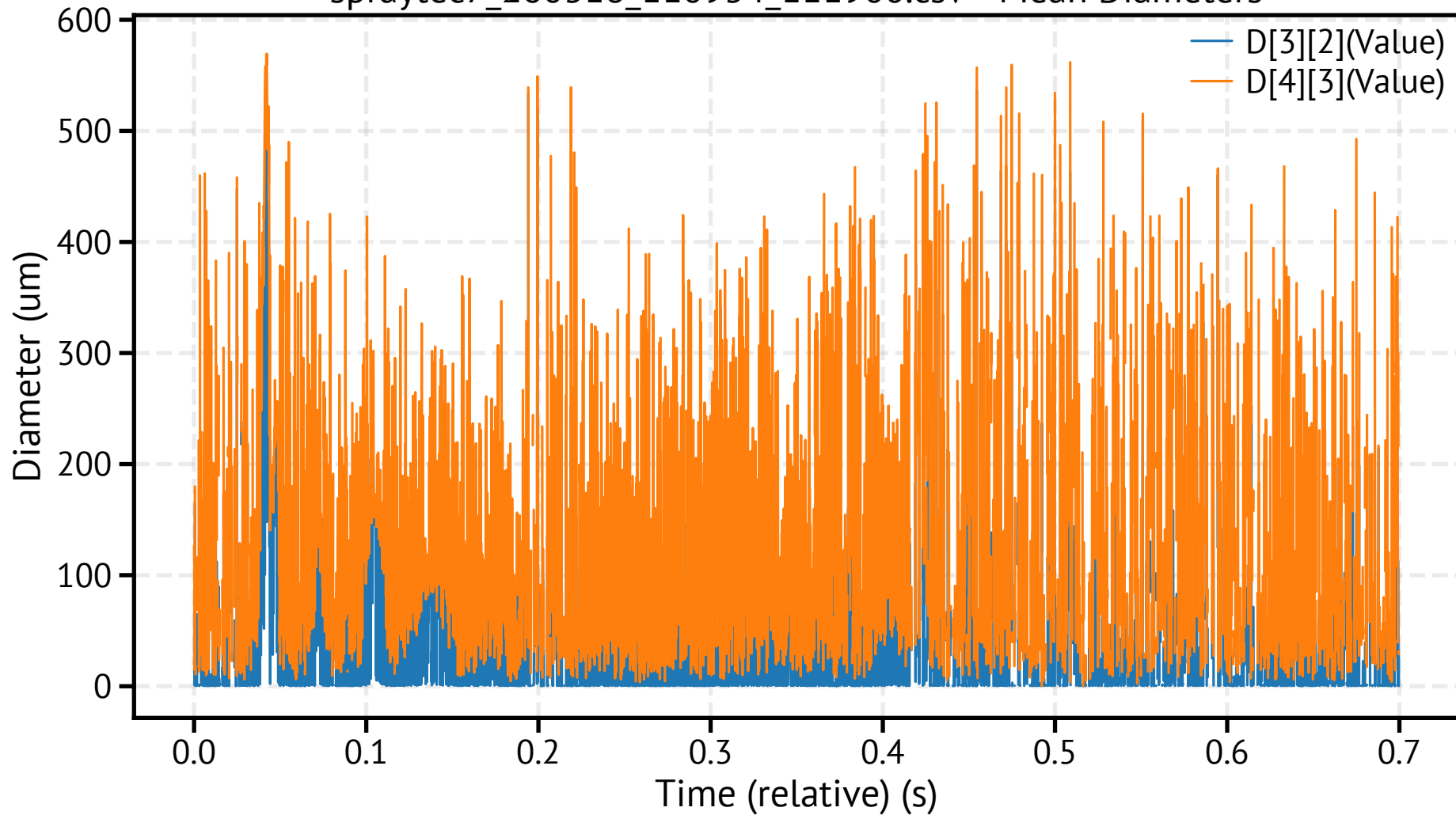
spraytec7_260318_110934_111900.csv - Mean Diameters
