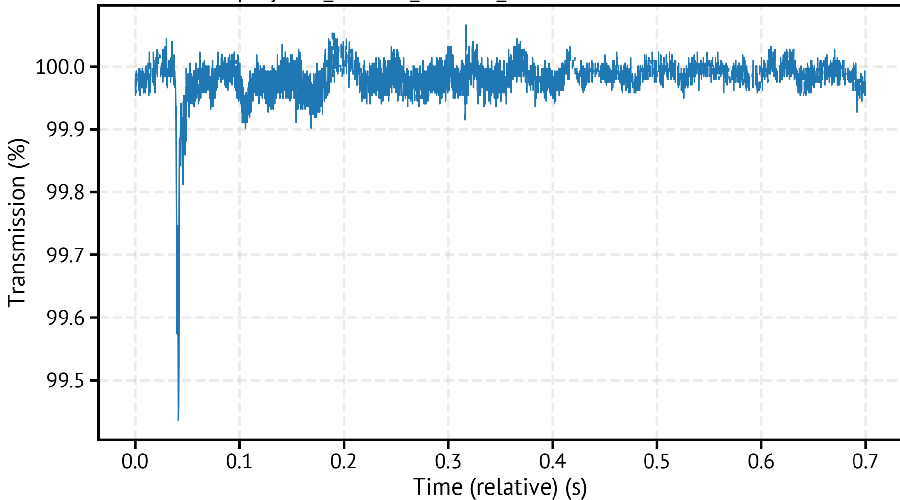
spraytec7_260318_110934_111900.csv - Transmission
