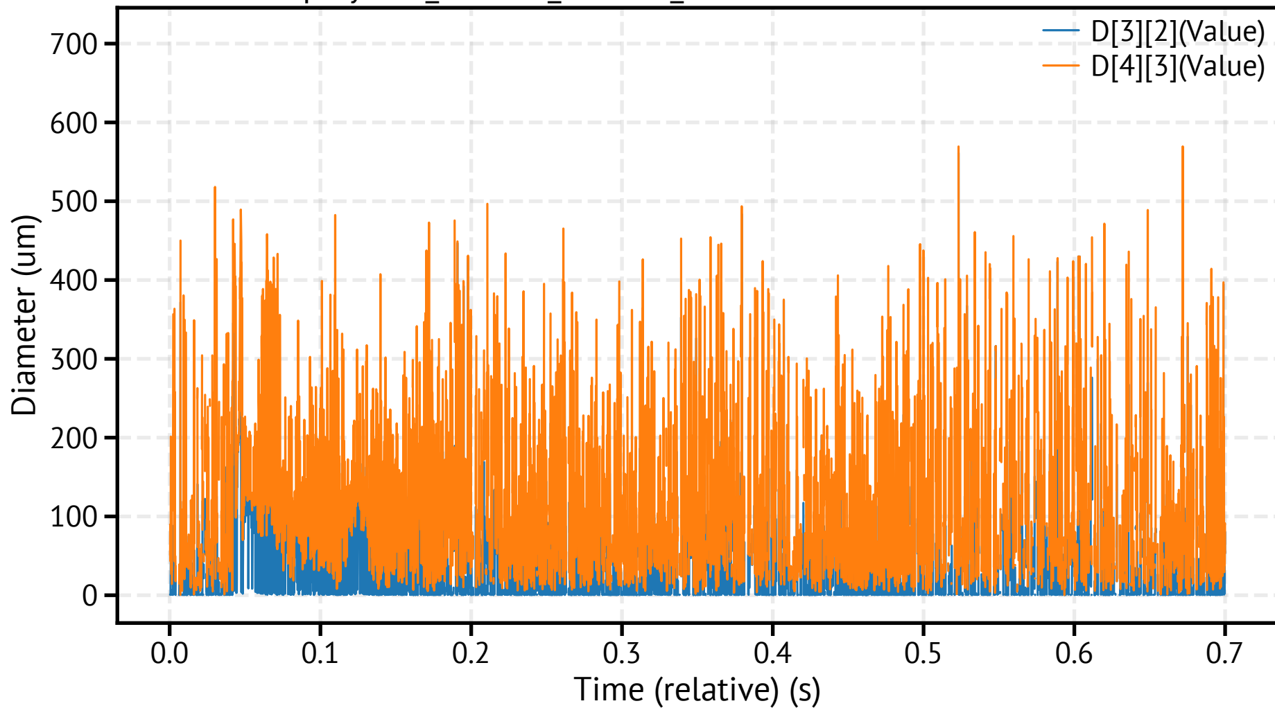
spraytec9_260318_111129_357700.csv - Mean Diameters
