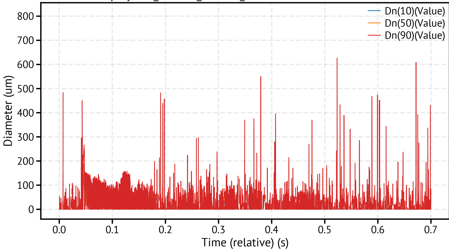
spraytec9_260318_111129_357700.csv - Dn Percentiles
