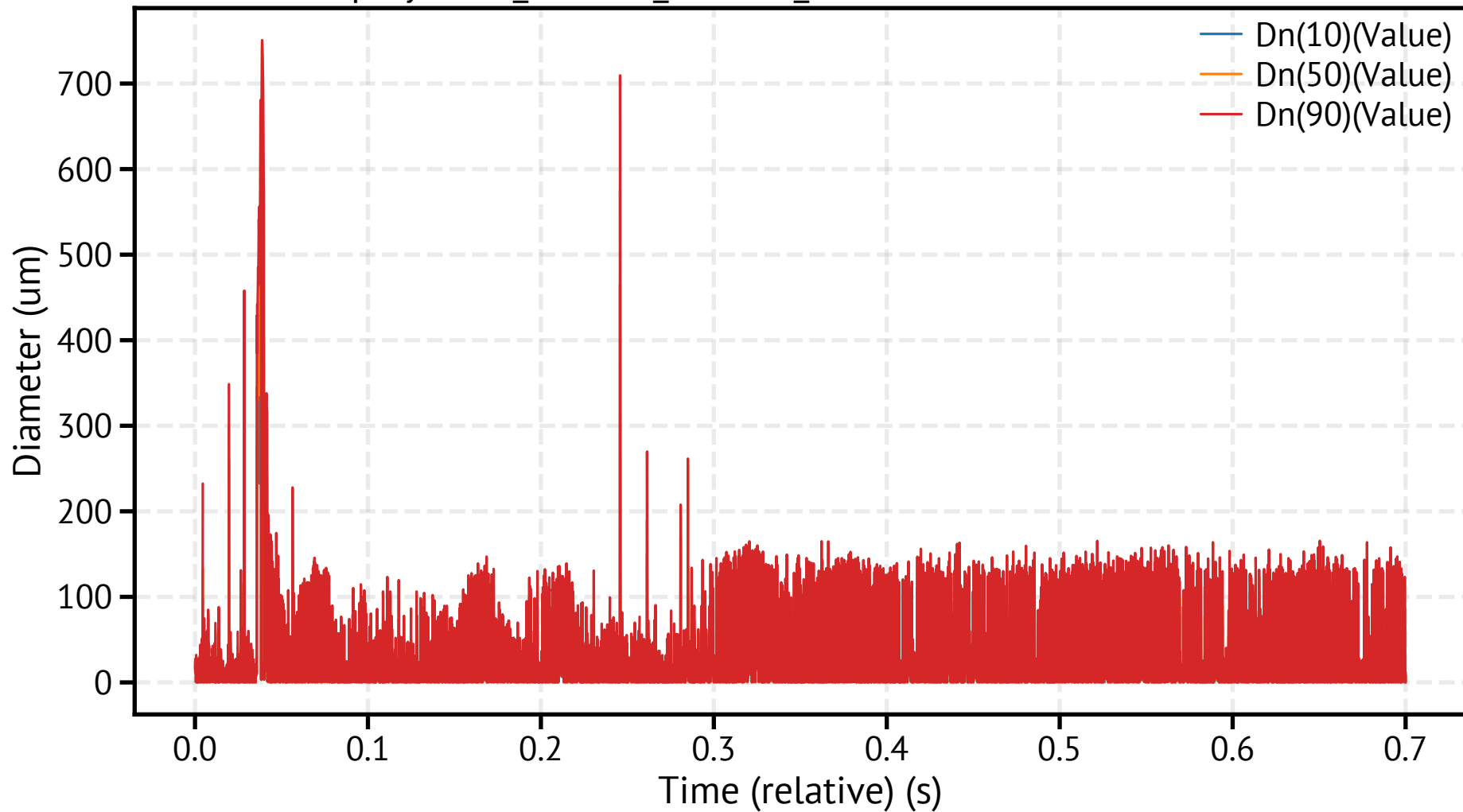
spraytec10_260318_112816_609500.csv - Dn Percentiles
