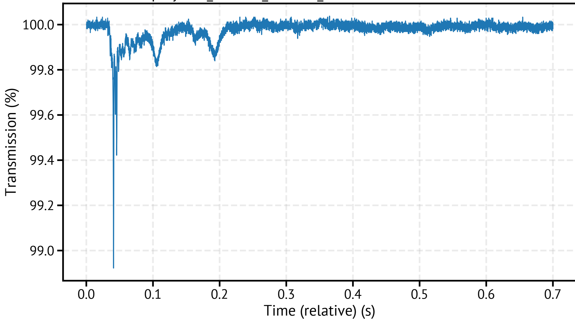
spraytec2_260318_112035_341900.csv - Transmission
