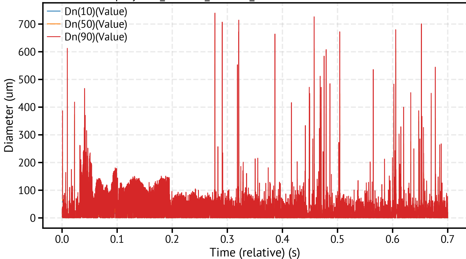
spraytec4_260318_112230_623100.csv - Dn Percentiles
