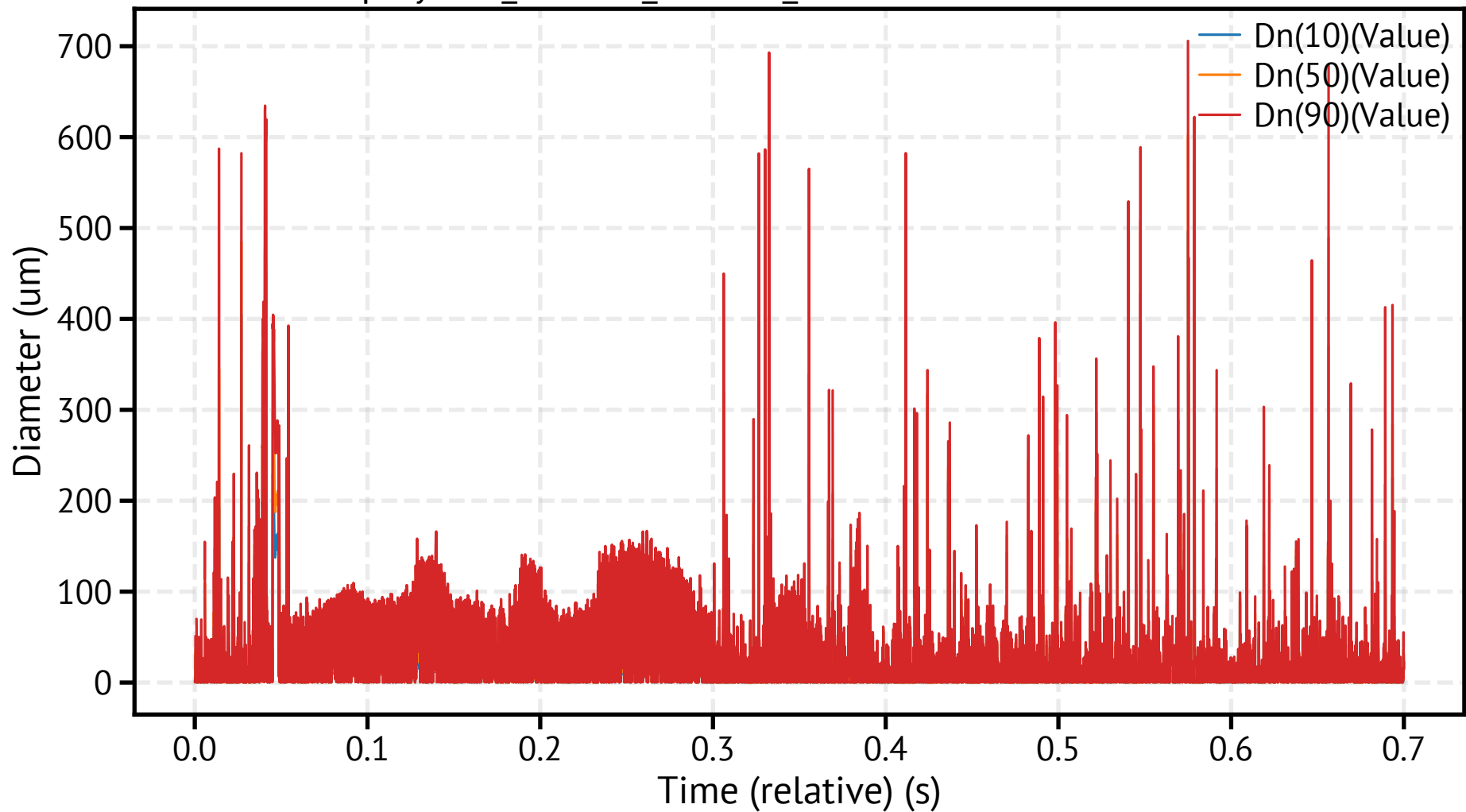
spraytec5_260318_112328_349400.csv - Dn Percentiles
