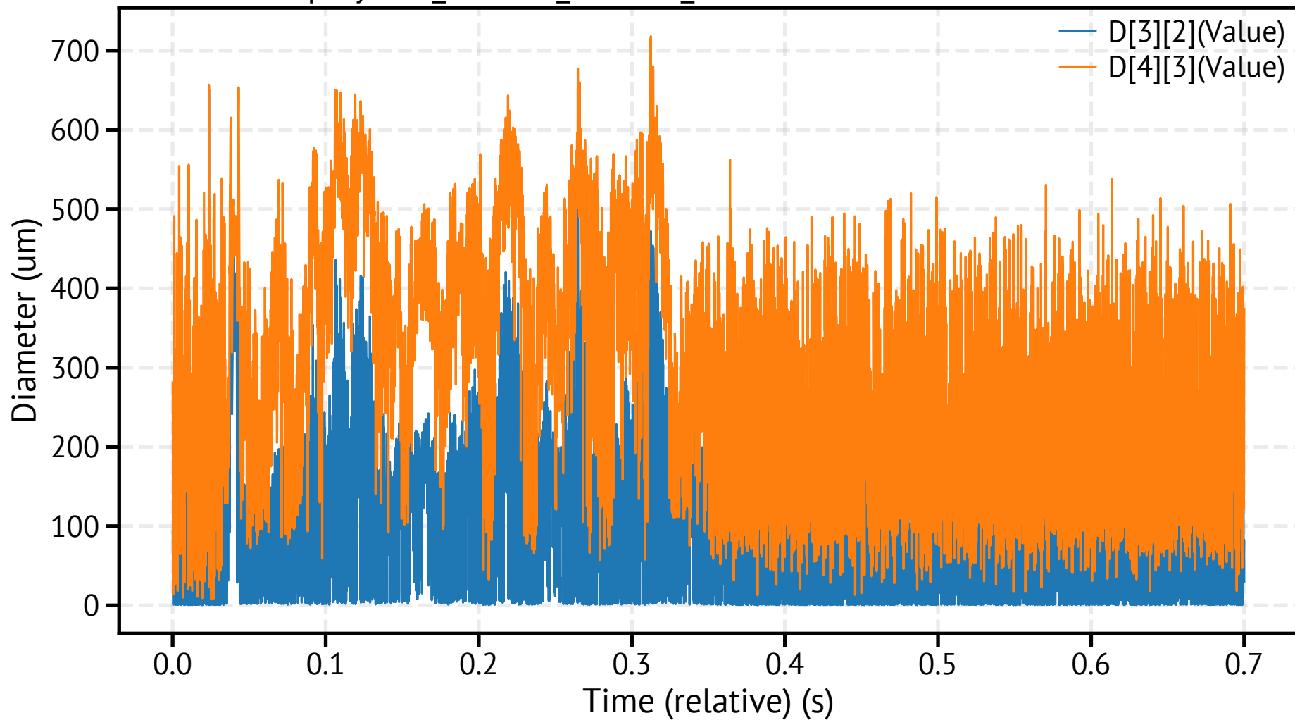
spraytec1_260318_113349_019700.csv - Mean Diameters
