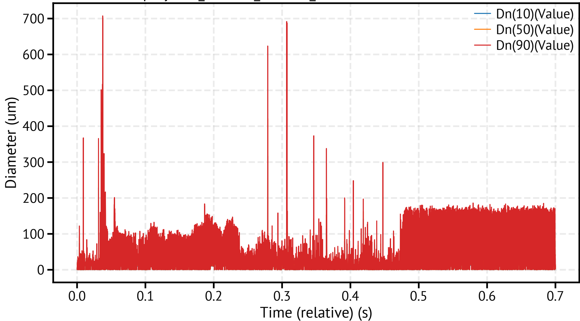
spraytec2_260318_113446_680200.csv - Dn Percentiles
