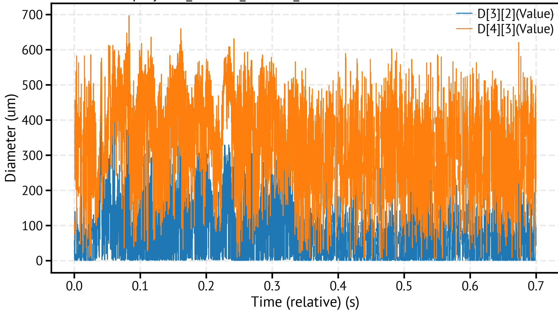
spraytec3_260318_113544_318000.csv - Mean Diameters
