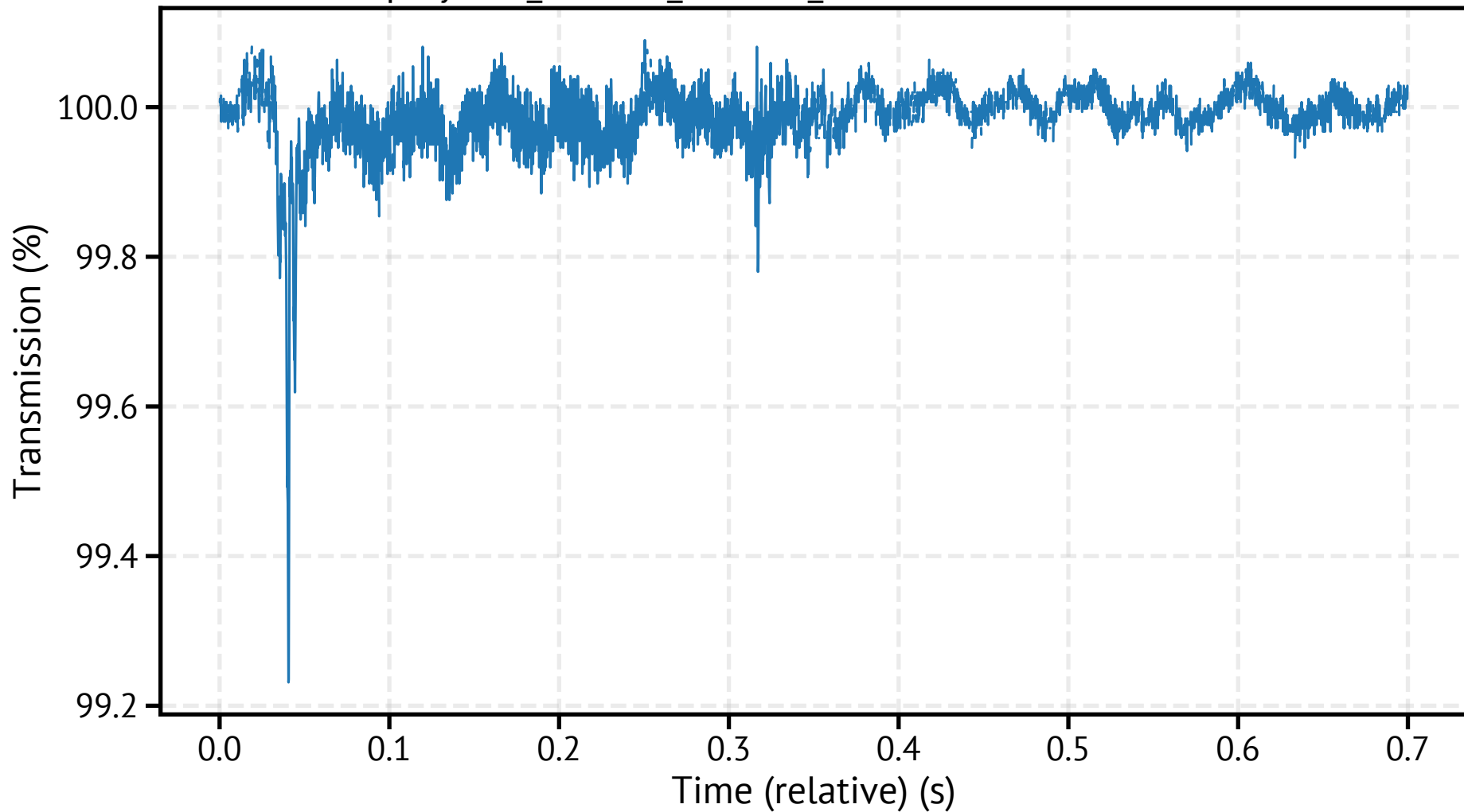
spraytec3_260318_113544_318000.csv - Transmission
