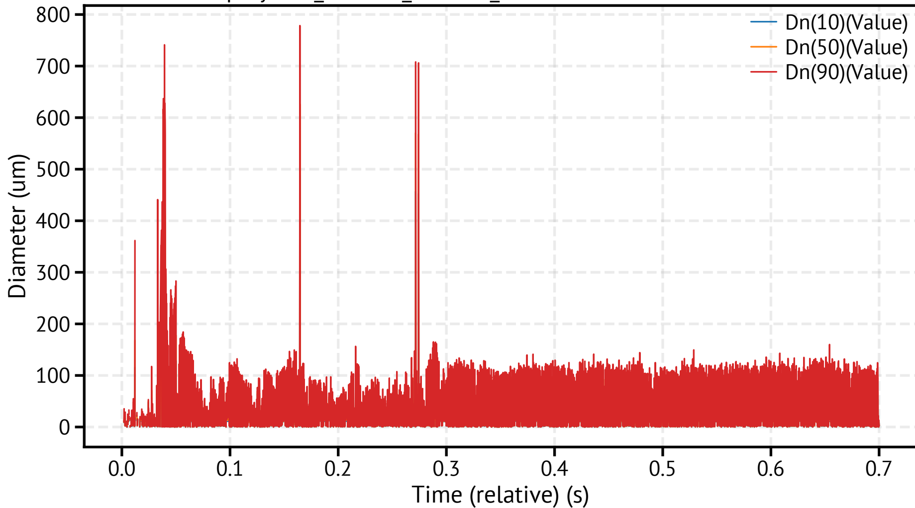
spraytec8_260318_114032_525900.csv - Dn Percentiles
