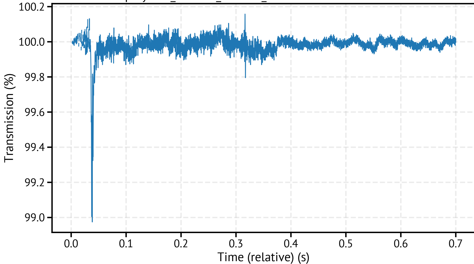
spraytec8_260318_114032_525900.csv - Transmission
