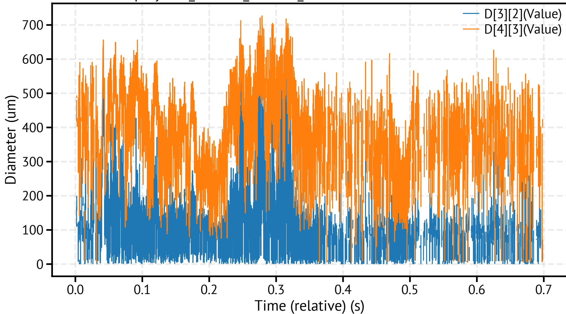
spraytec9_260318_114130_216500.csv - Mean Diameters
