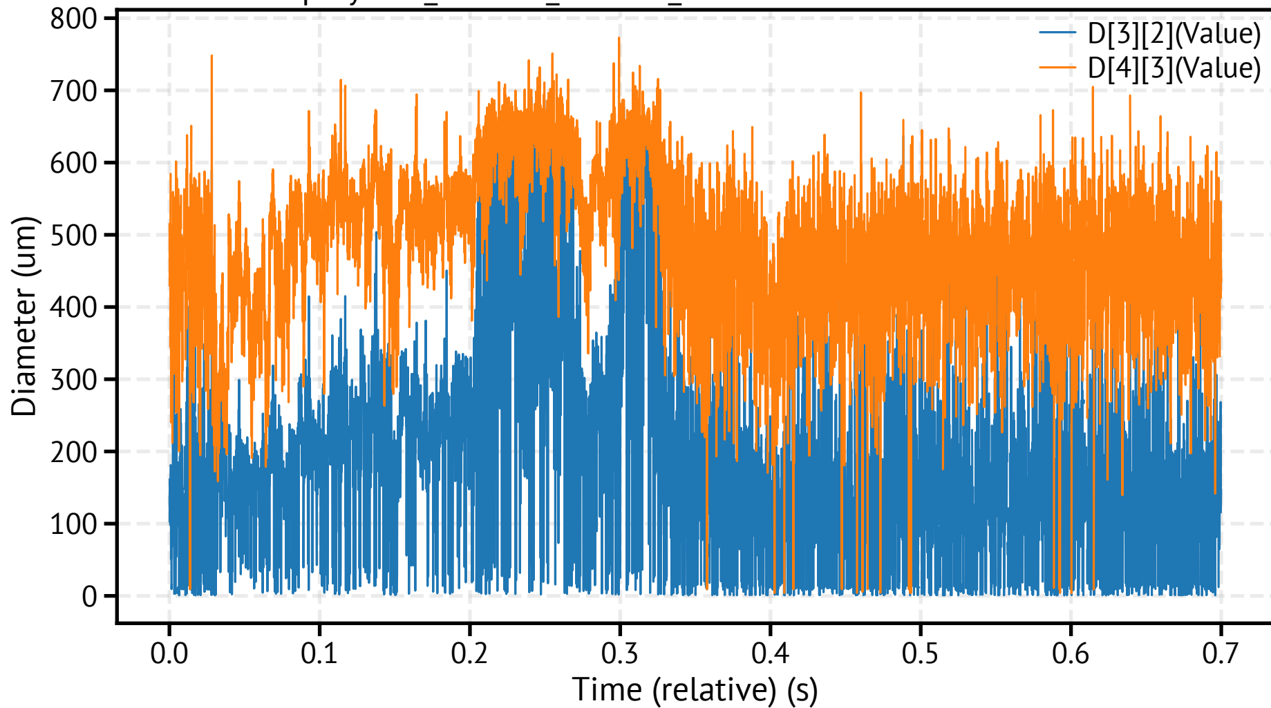
spraytec3_260318_115049_401500.csv - Mean Diameters
