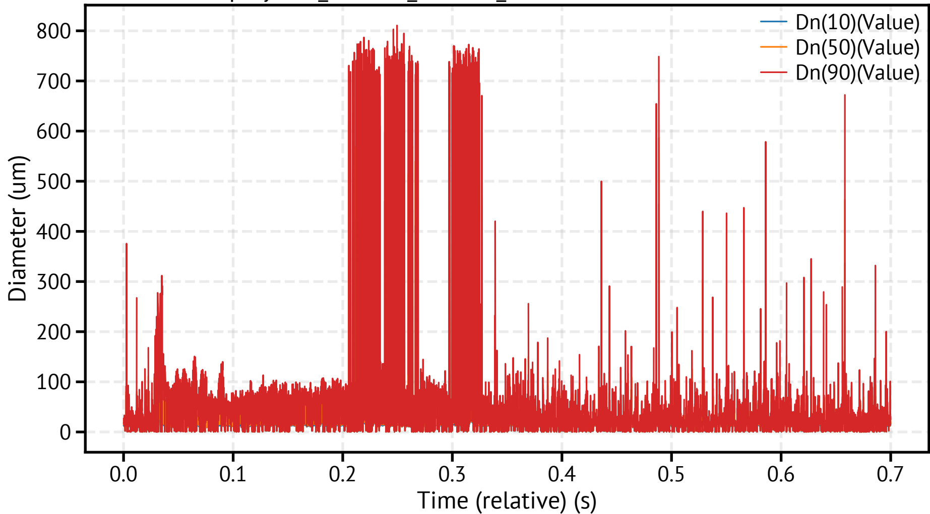
spraytec3_260318_115049_401500.csv - Dn Percentiles
