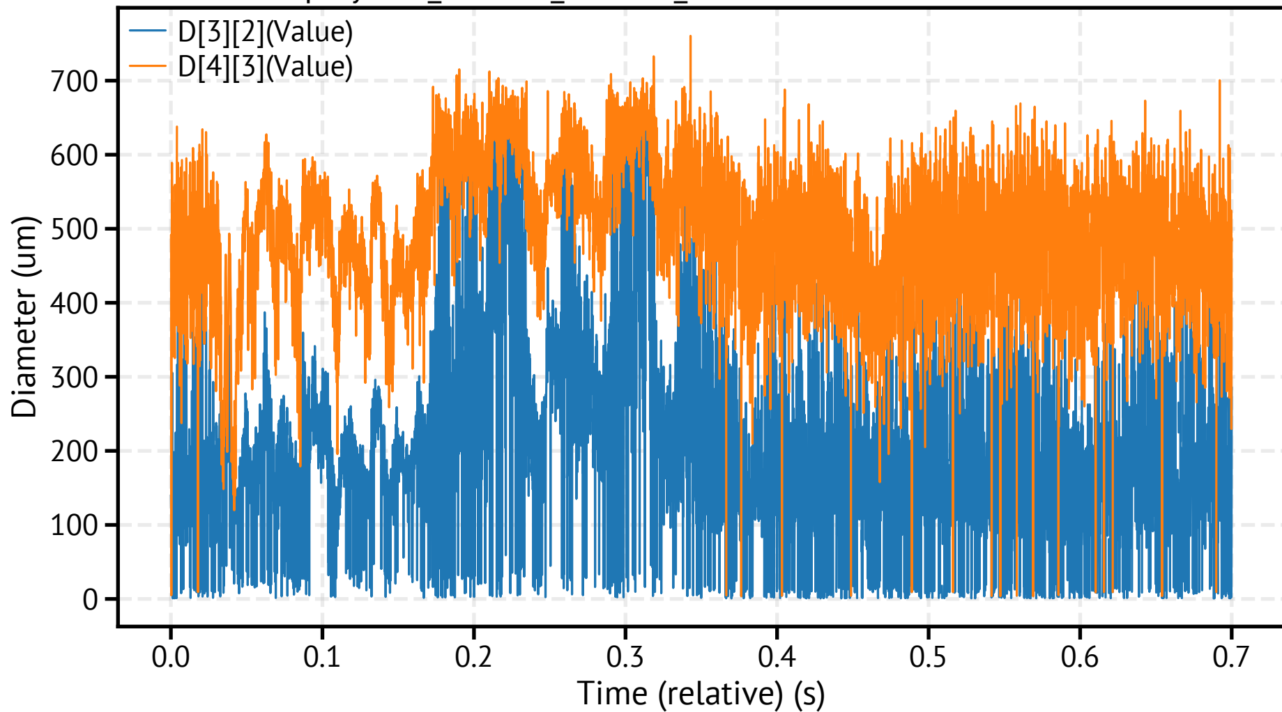
spraytec6_260318_115342_353900.csv - Mean Diameters
