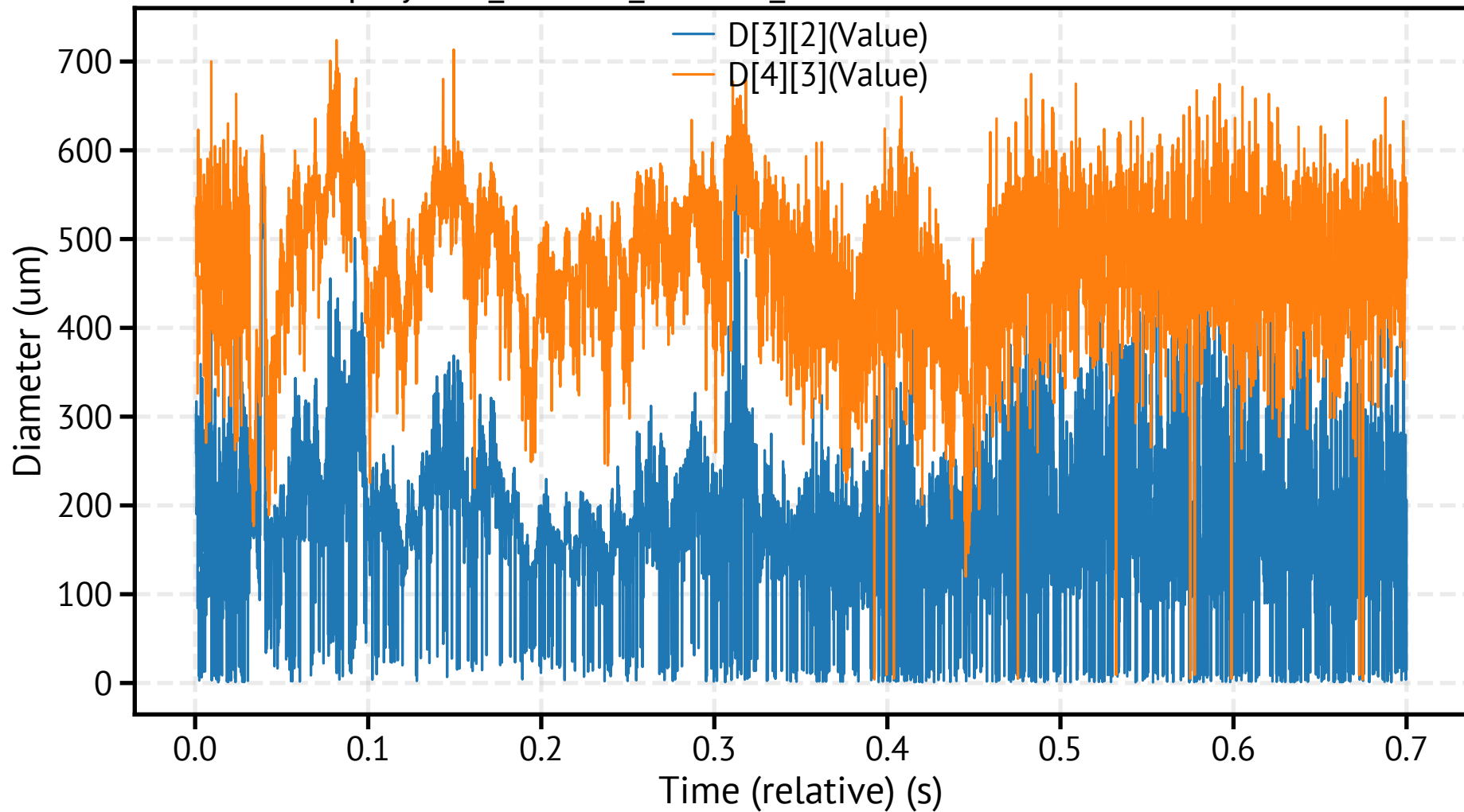
spraytec7_260318_115440_025200.csv - Mean Diameters
