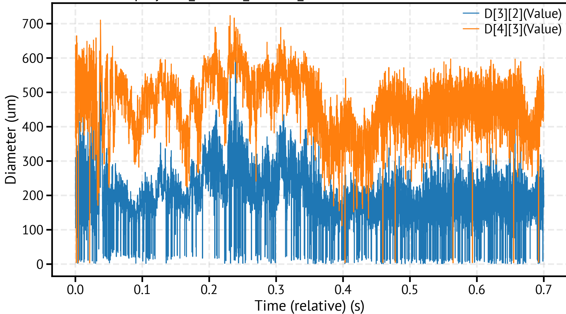
spraytec8_260318_115537_667200.csv - Mean Diameters
