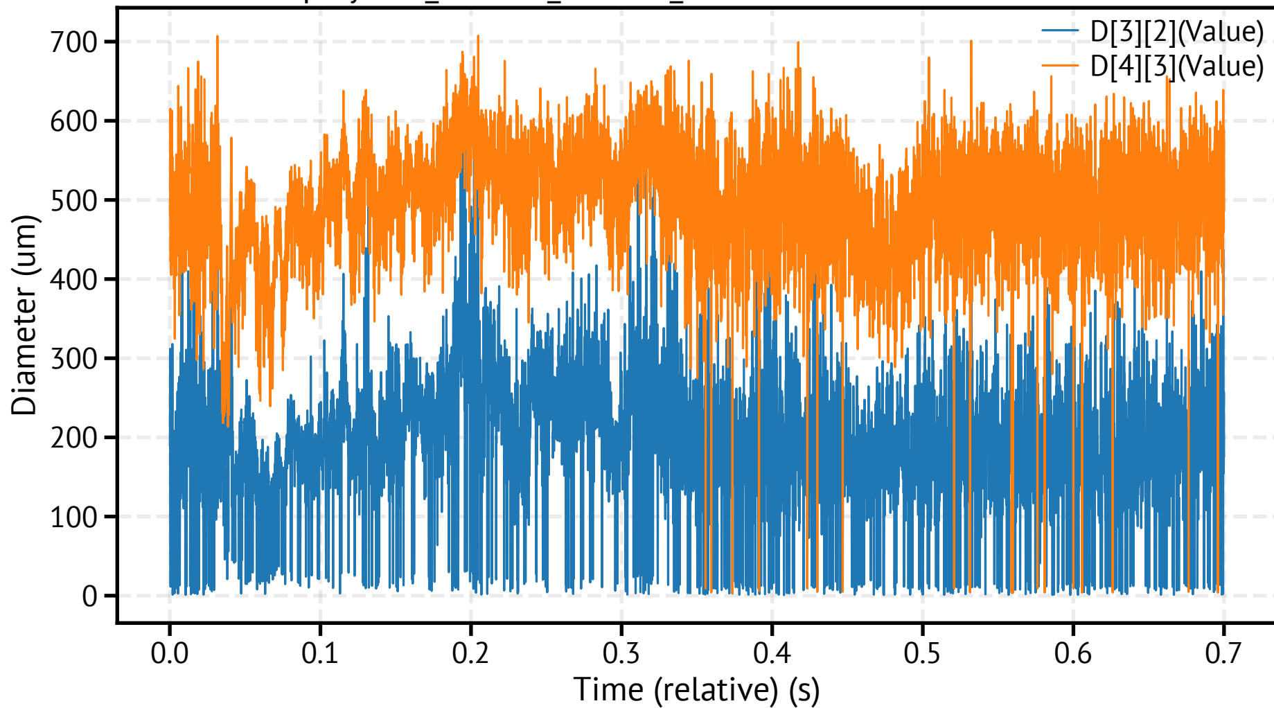
spraytec9_260318_115635_296800.csv - Mean Diameters
