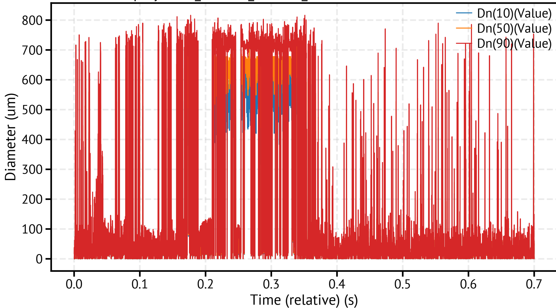
spraytec10_260318_121629_528900.csv - Dn Percentiles
