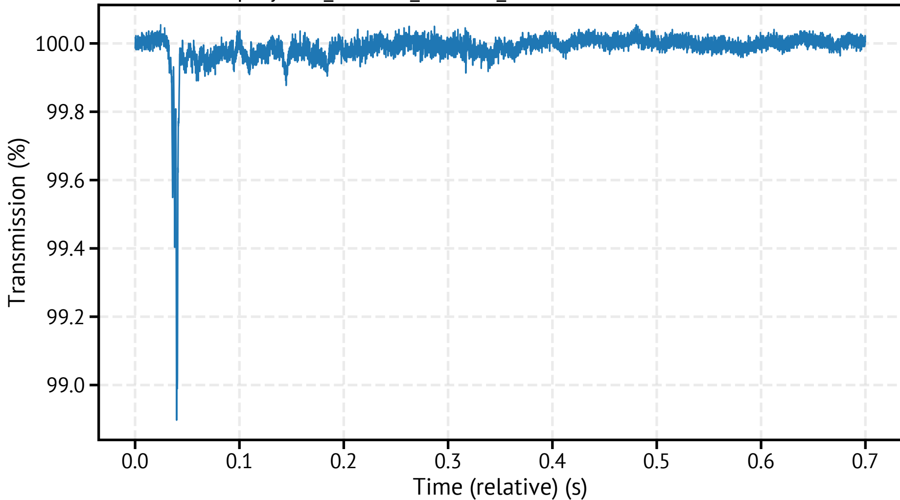
spraytec2_260318_120848_000900.csv - Transmission
