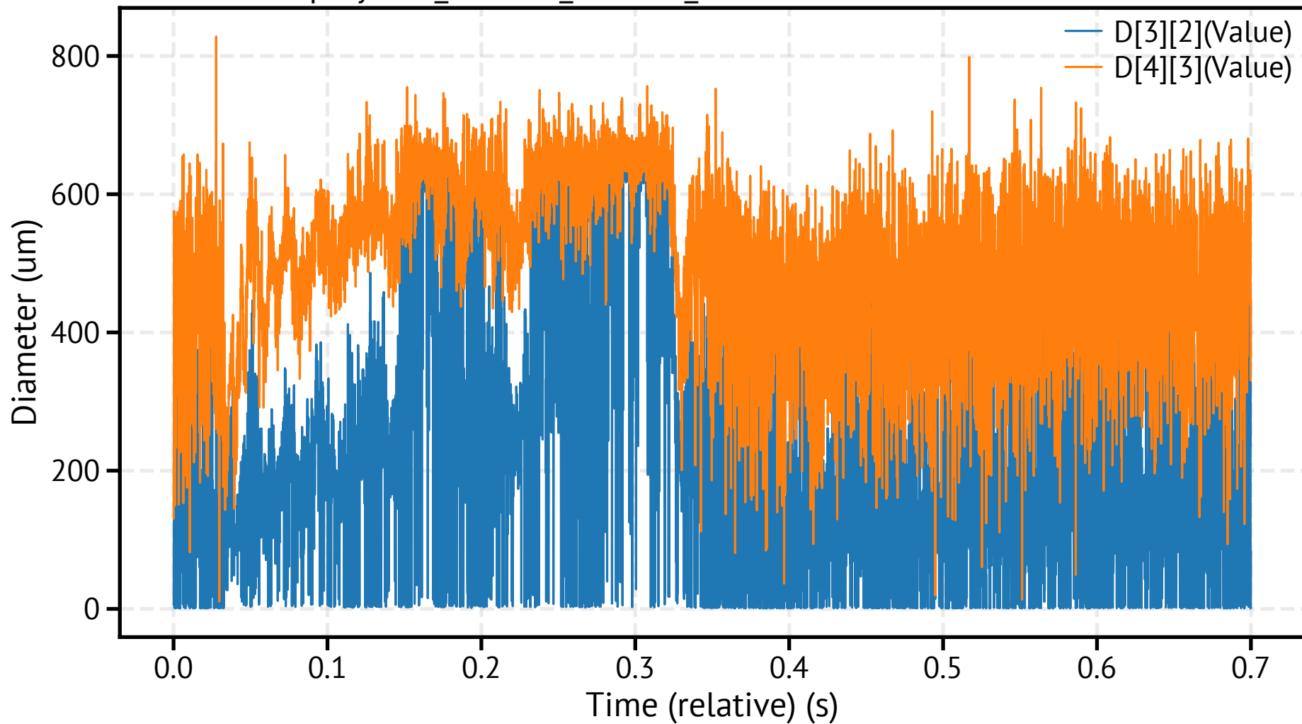
spraytec4_260318_121043_538400.csv - Mean Diameters
