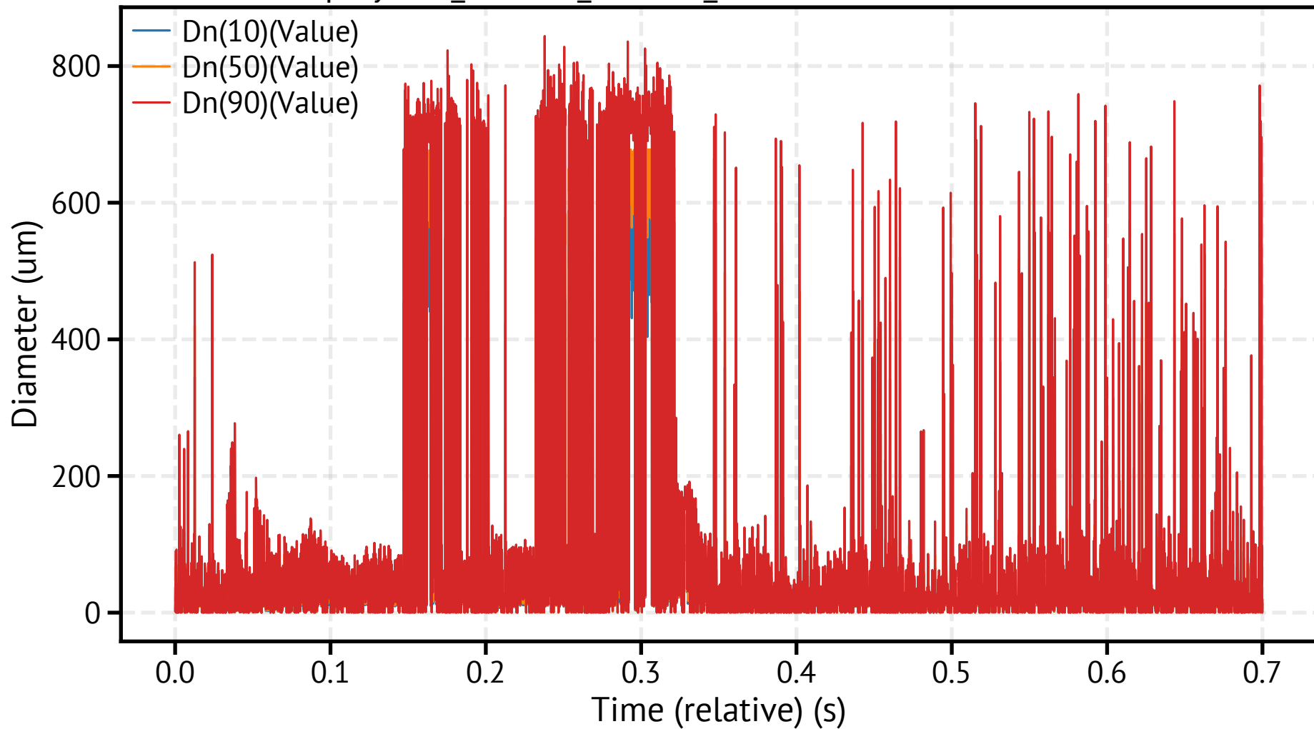
spraytec4_260318_121043_538400.csv - Dn Percentiles
