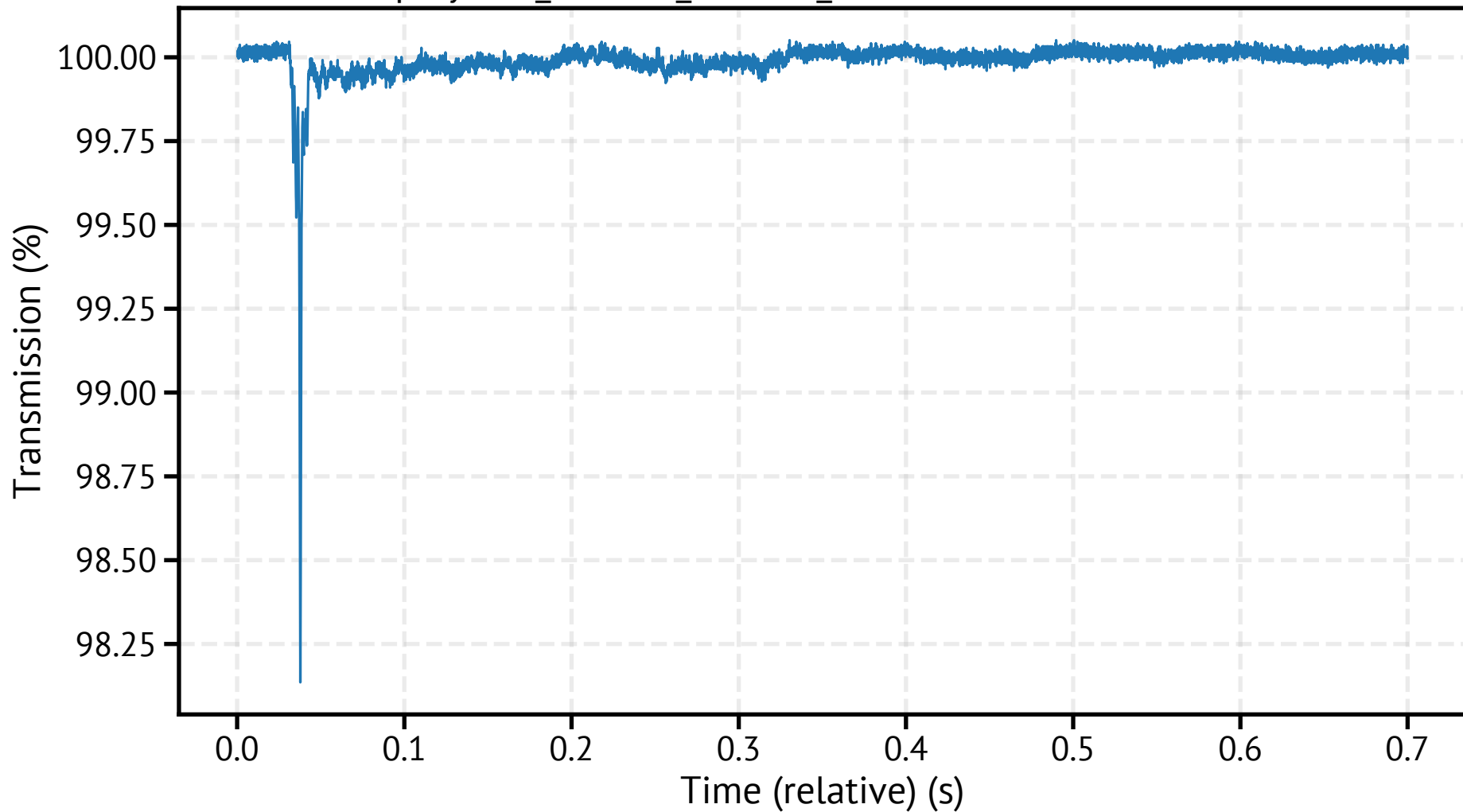
spraytec5_260318_121141_072000.csv - Transmission
