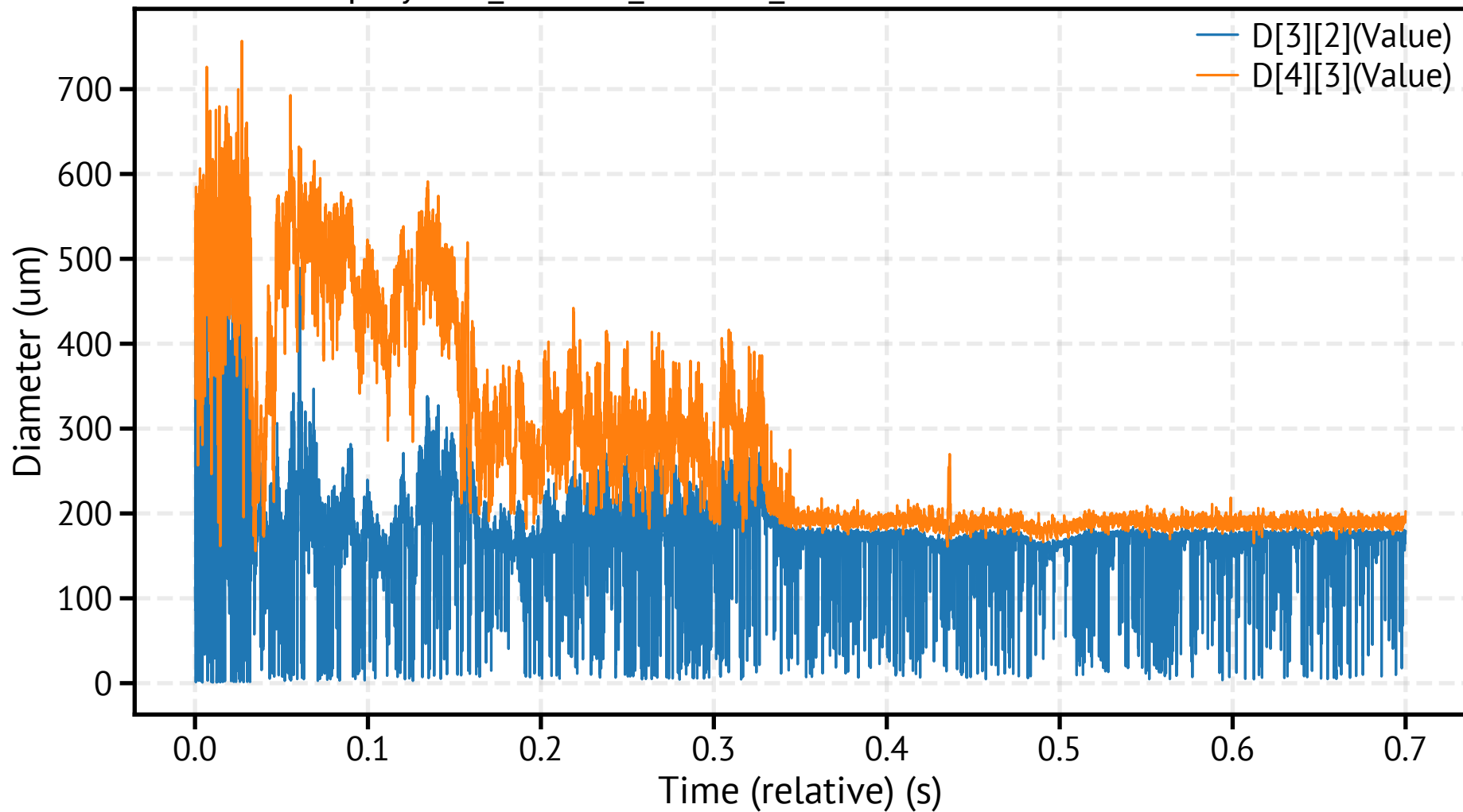
spraytec6_260318_121238_869200.csv - Mean Diameters
