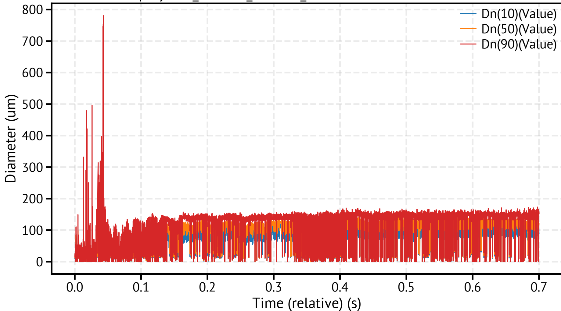
spraytec7_260318_121336_590200.csv - Dn Percentiles
