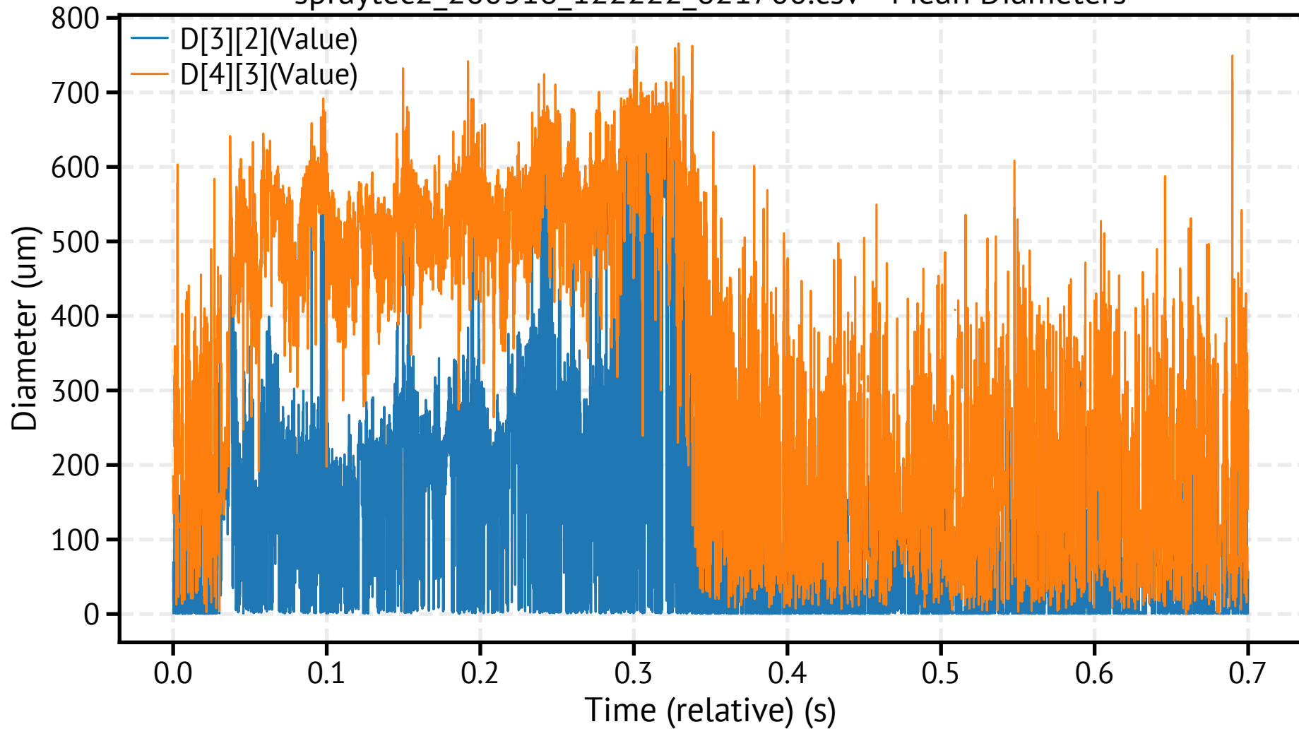
spraytec2_260318_122222_821700.csv - Mean Diameters
