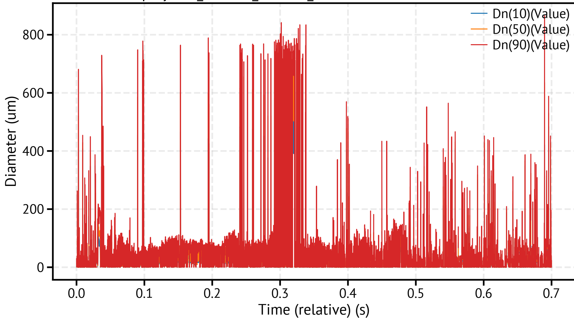
spraytec2_260318_122222_821700.csv - Dn Percentiles
