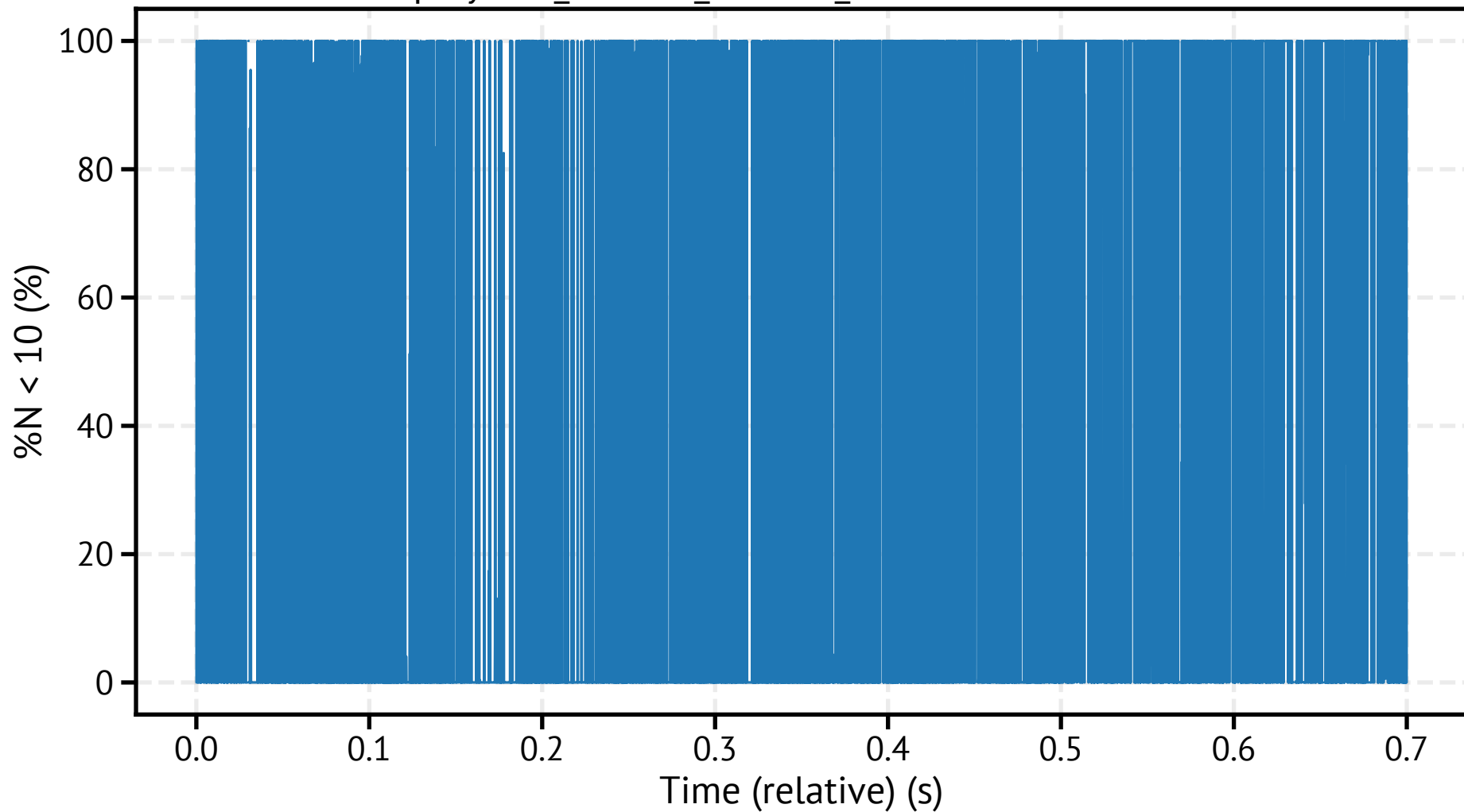
spraytec2_260318_122222_821700.csv - %N < 10
