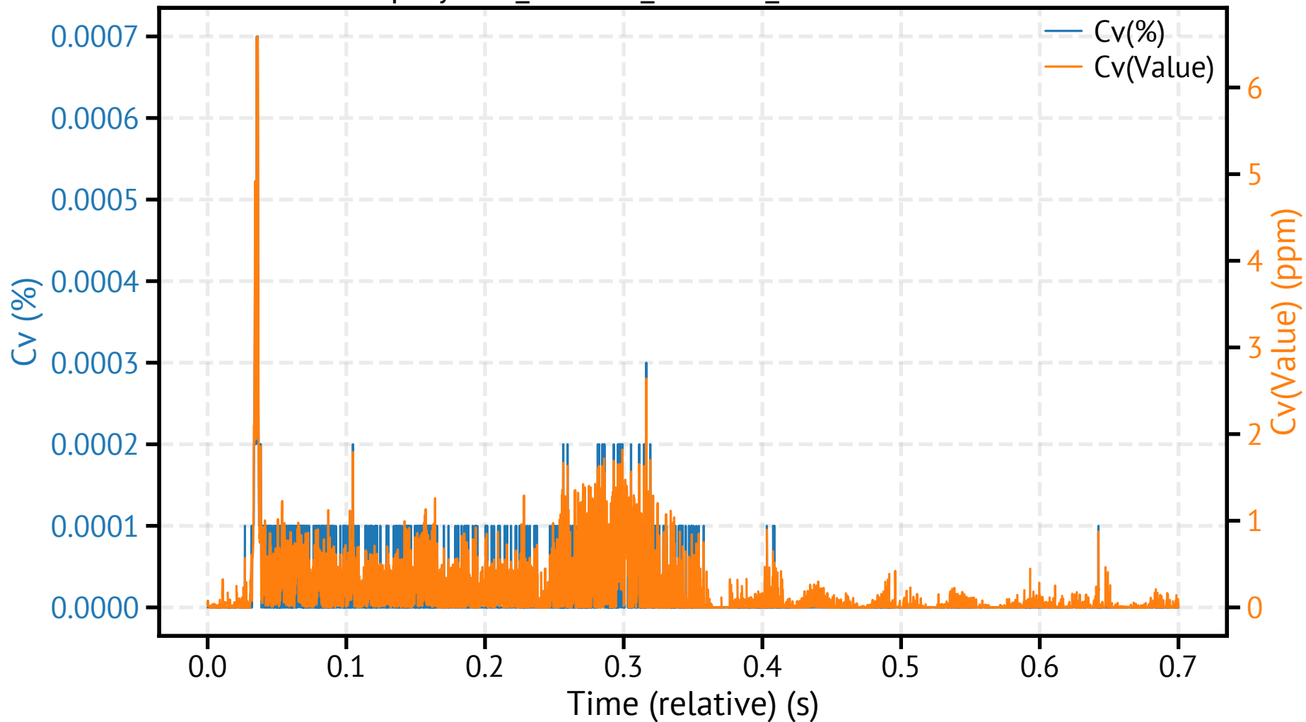
spraytec3_260318_122320_395100.csv - Cv
