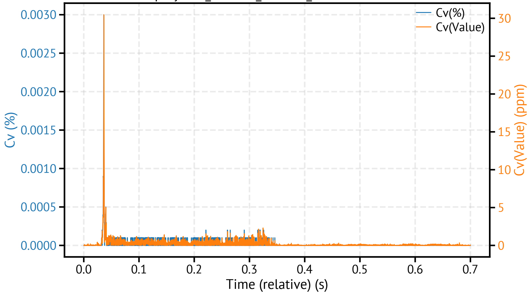
spraytec4_260318_122418_142300.csv - Cv
