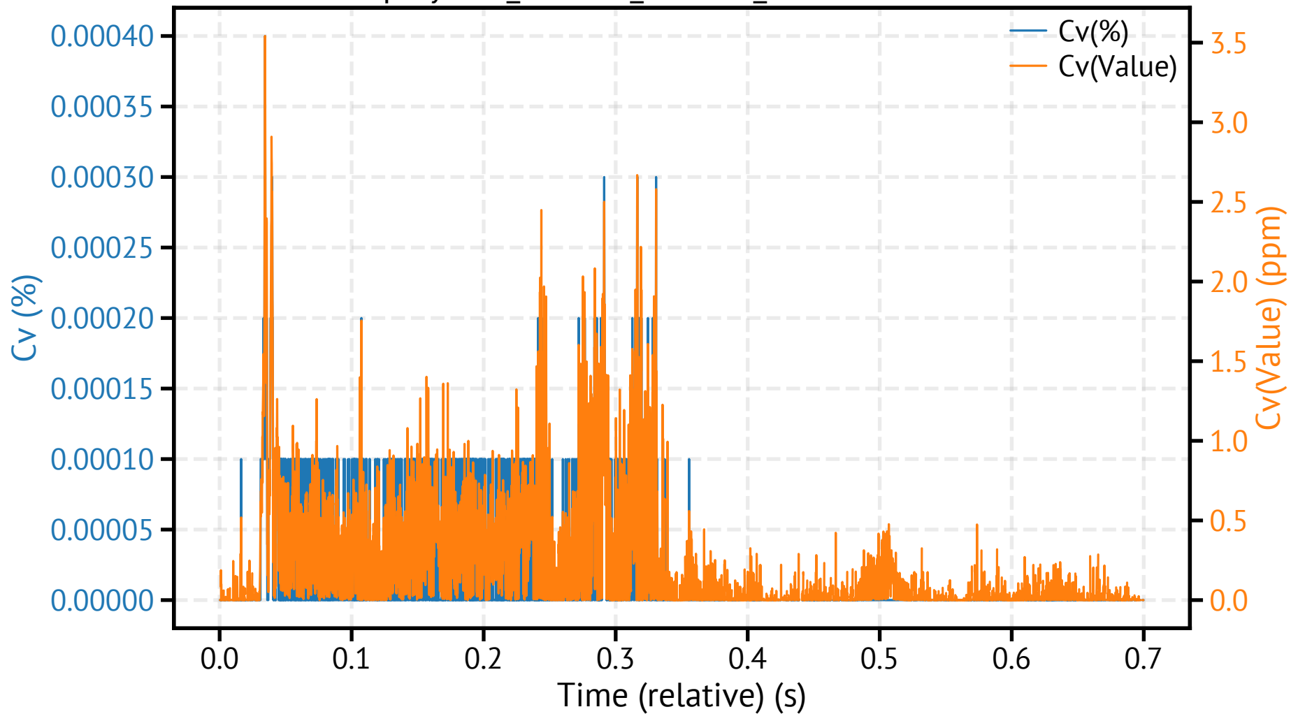
spraytec5_260318_122515_895900.csv - Cv
