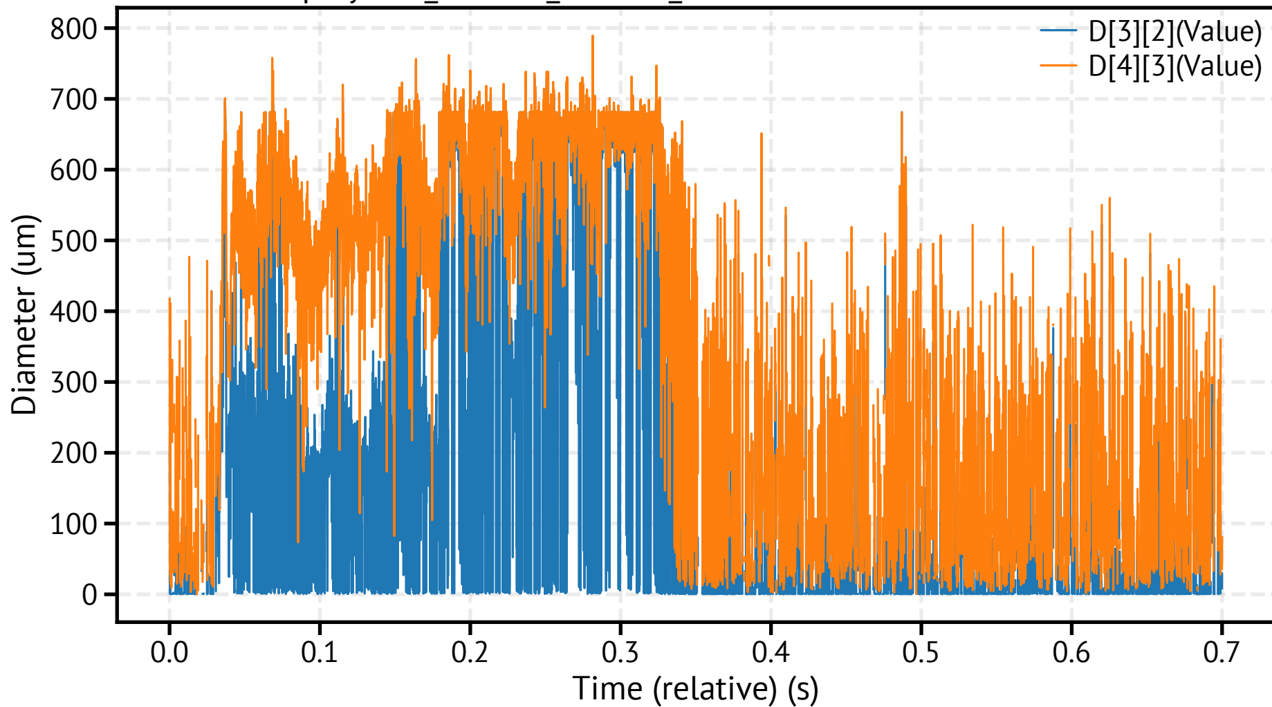
spraytec7_260318_122711_236800.csv - Mean Diameters
