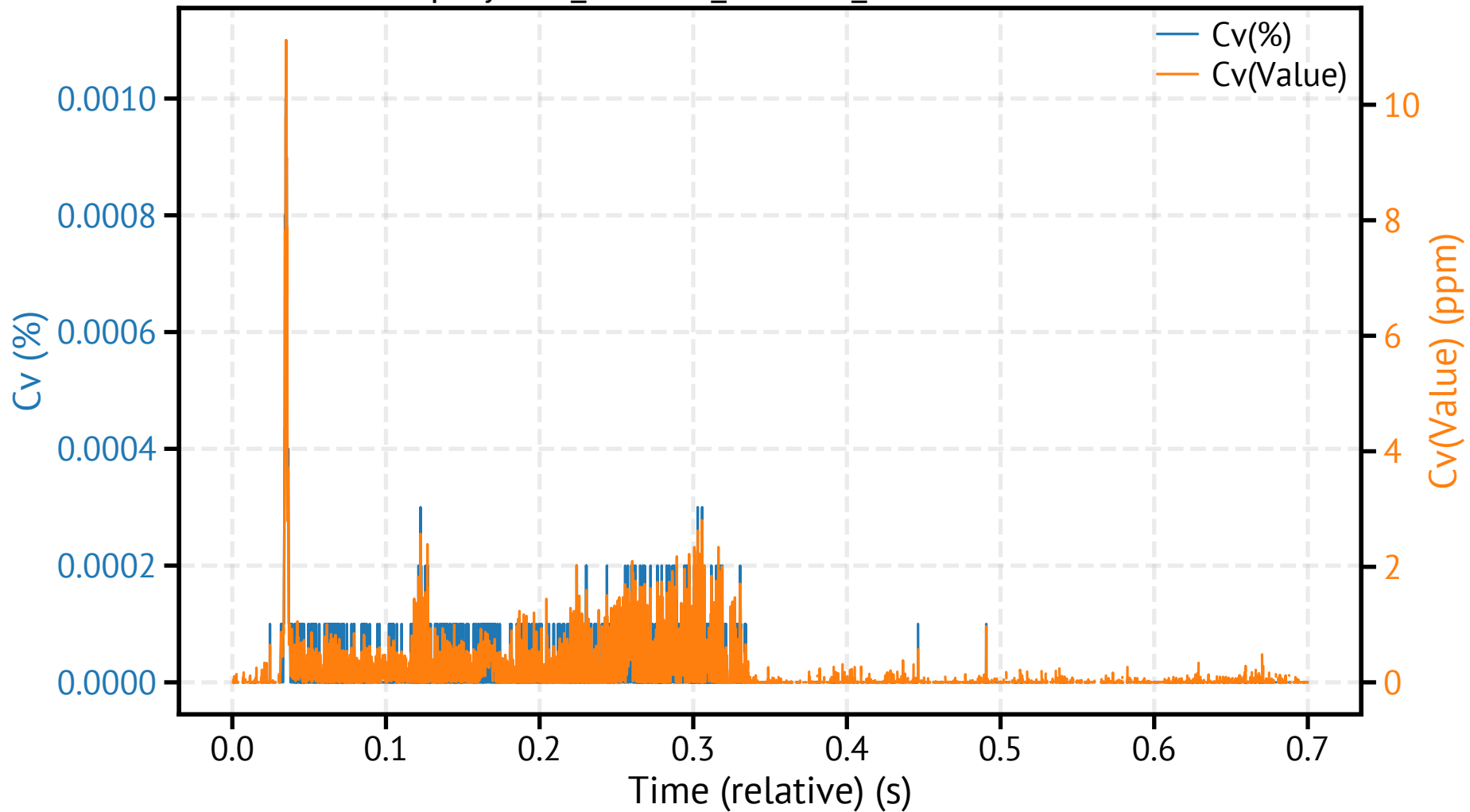
spraytec8_260318_122808_794200.csv - Cv
