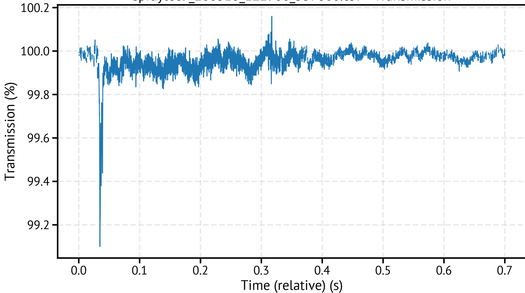
spraytec9_260318_122906_537800.csv - Transmission
