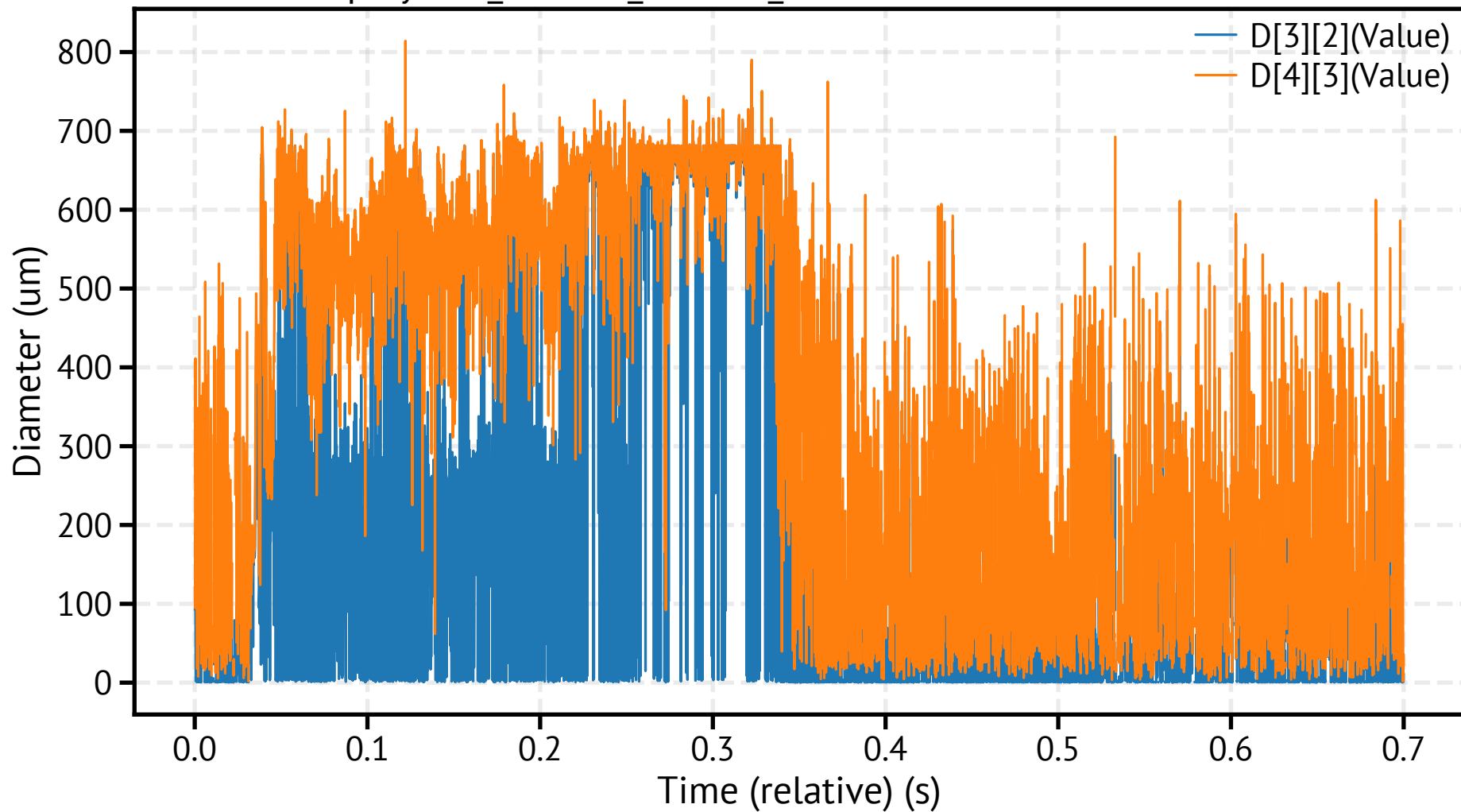
spraytec1_260318_135319_165400.csv - Mean Diameters
