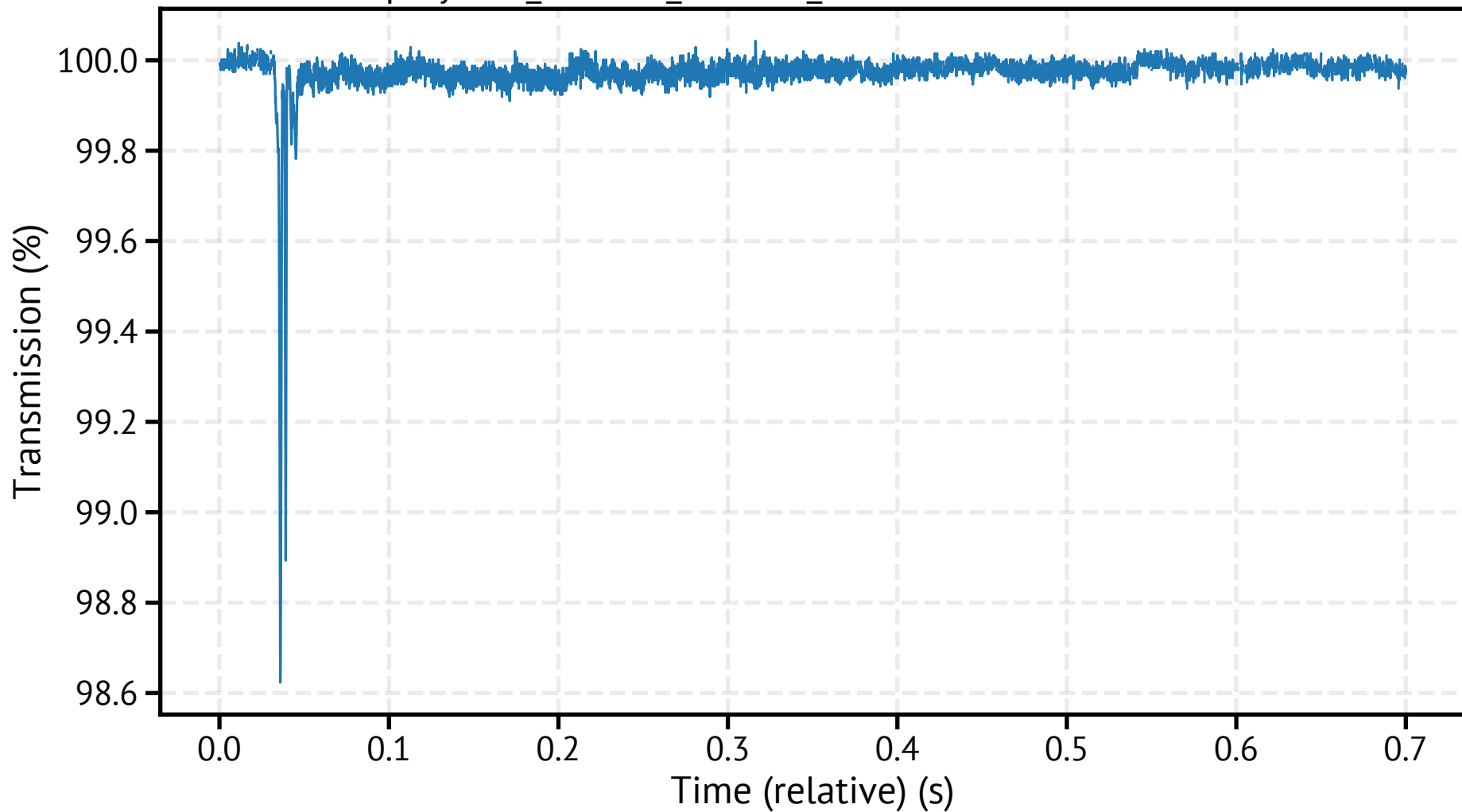
spraytec1_260318_135319_165400.csv - Transmission
